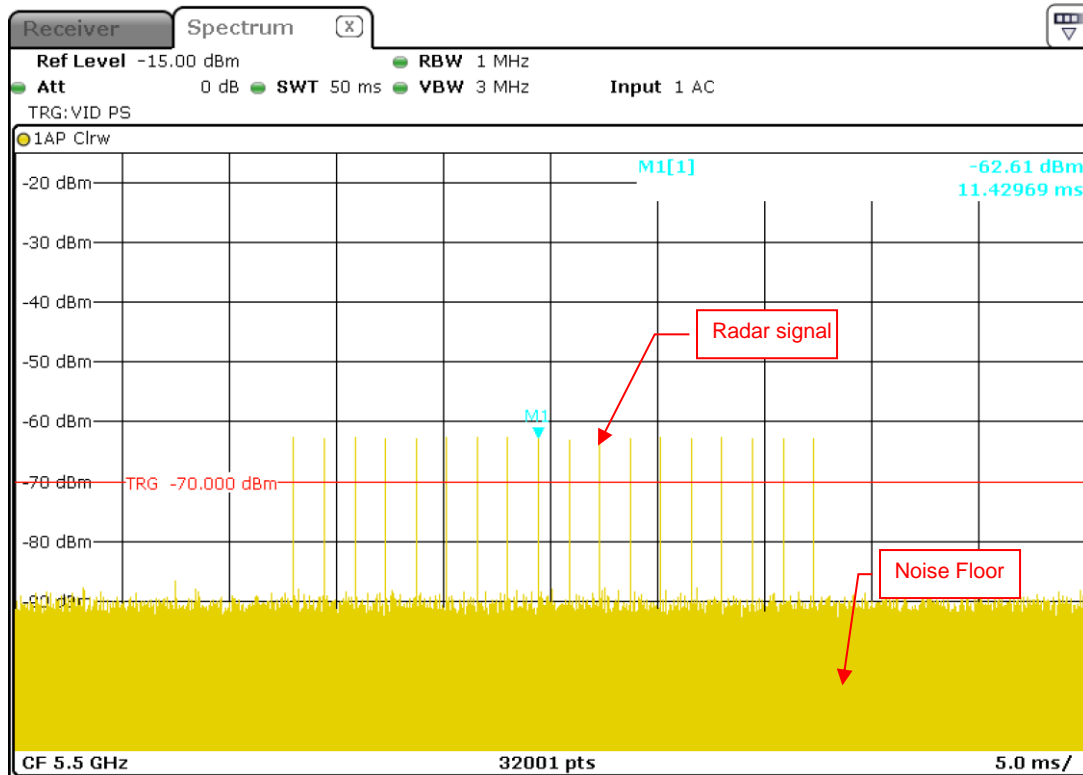
Radar Signal 0
