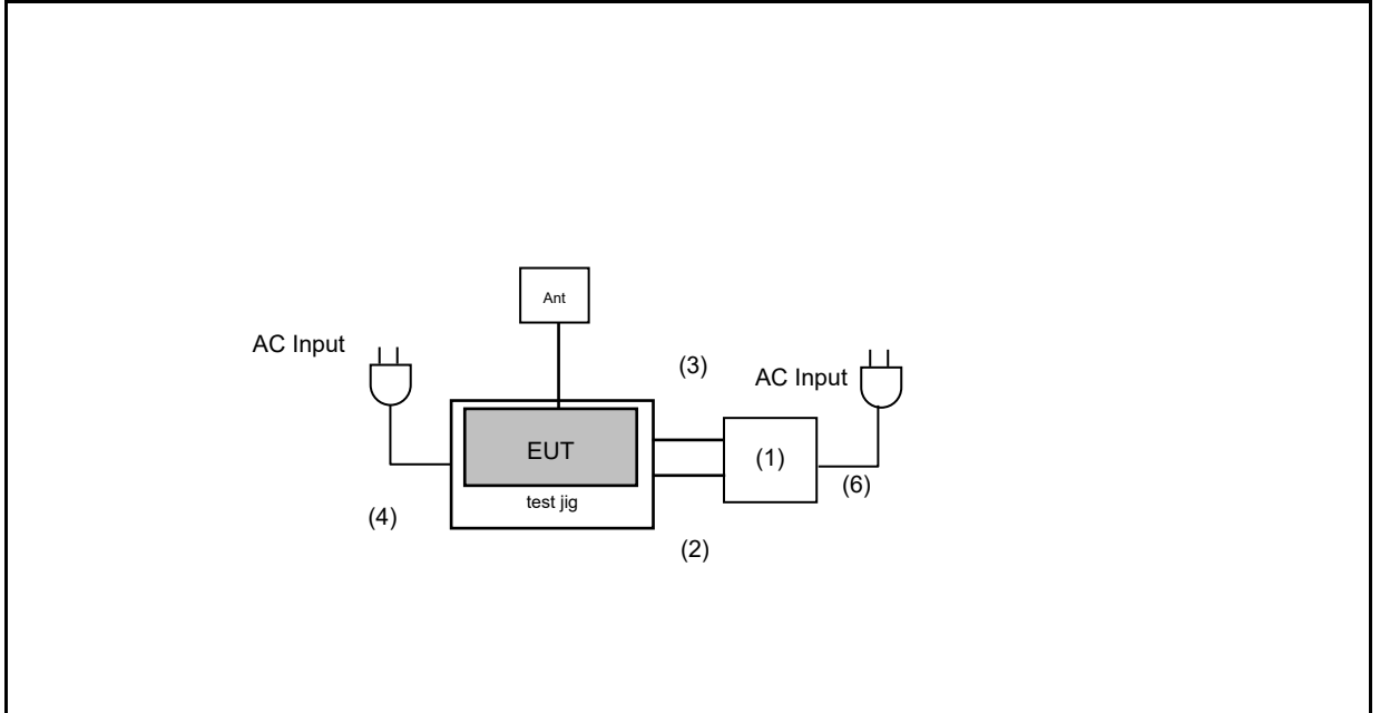
Radiated Emission(Below 1 GHz & Conduction Emission)
