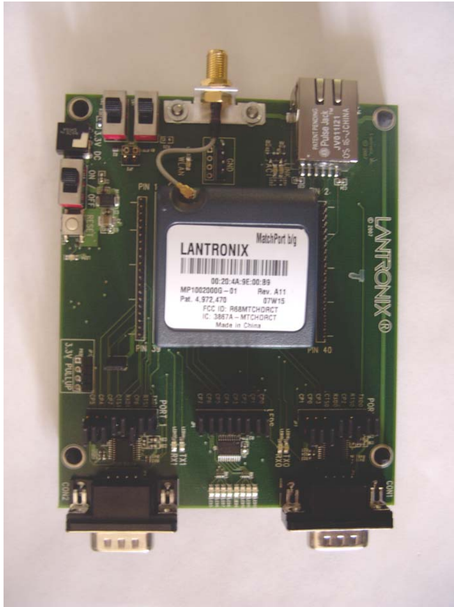
Board Top View
