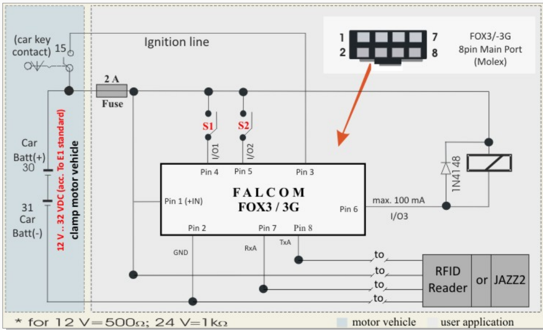
Figure 29: Schematic example of installation guidance.
