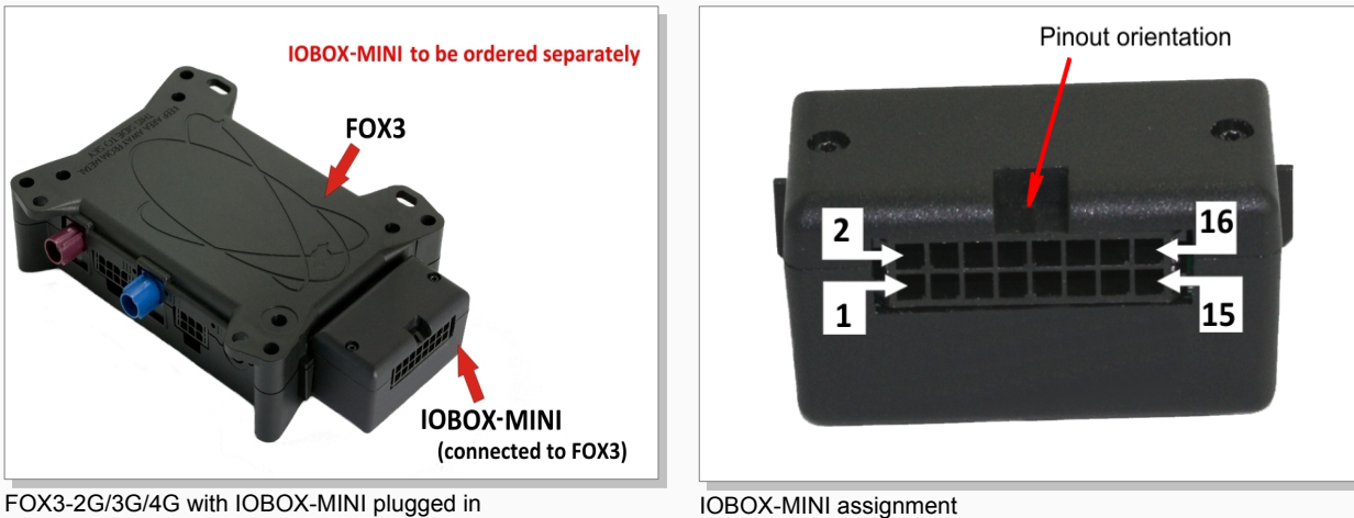
Figure 23: IOBOX-MINI pinout.
