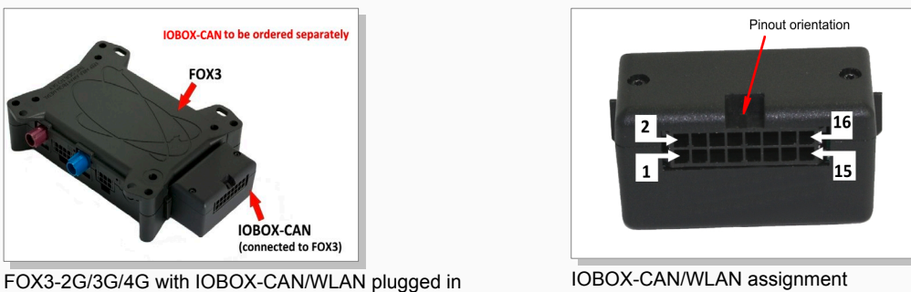
Figure 24: IOBOX-CAN/WLAN pinout.
