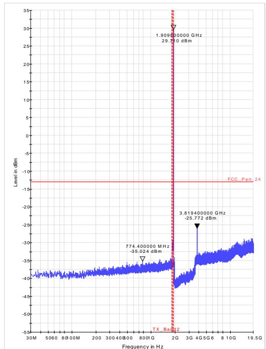
Diagram 36.31_RSE_Ch810_EGPRS_Sweep2
