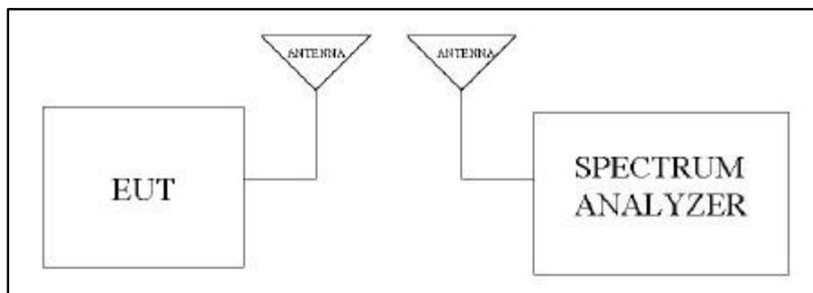
Figure A-1. Test Instrument & Measurement Setup
