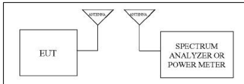
Figure A-3. Test Instrument & Measurement Setup
