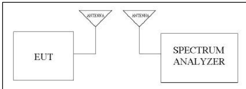
Figure A-2. Test Instrument & Measurement Setup
