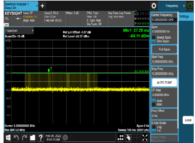
VHT80_5290MHz_Radar_Type 1-B
