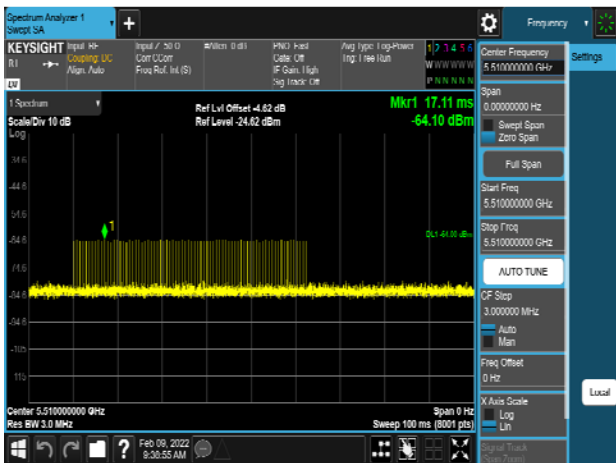
HT40_5510MHz_Radar_Type 1-B
