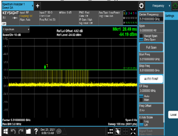
HT40_5510MHz_Radar_Type 1-B
