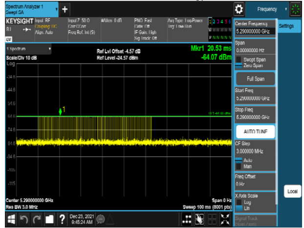
VHT80_5290MHz_Radar_Type 1-B
