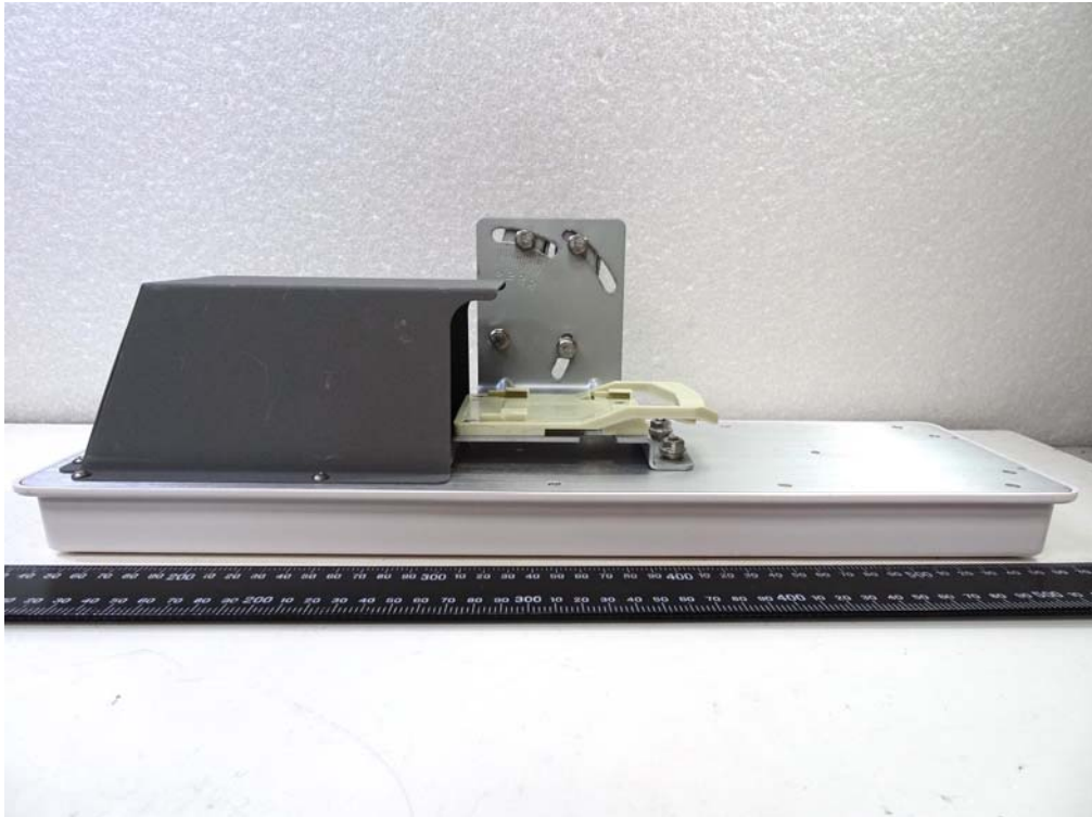
Side View – 4
