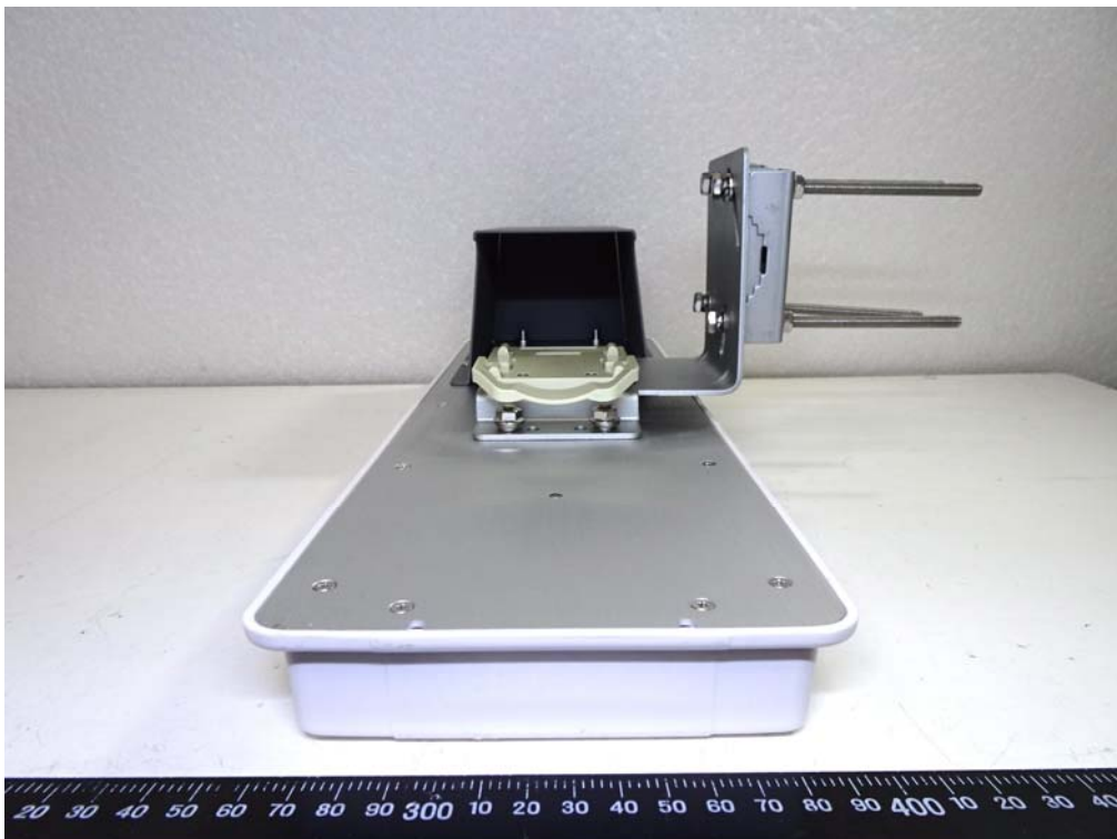
Side View – 4
