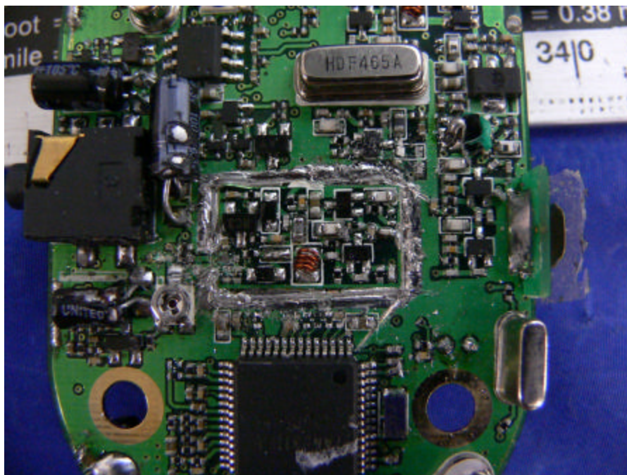
EUT – Solder View Shield off View
