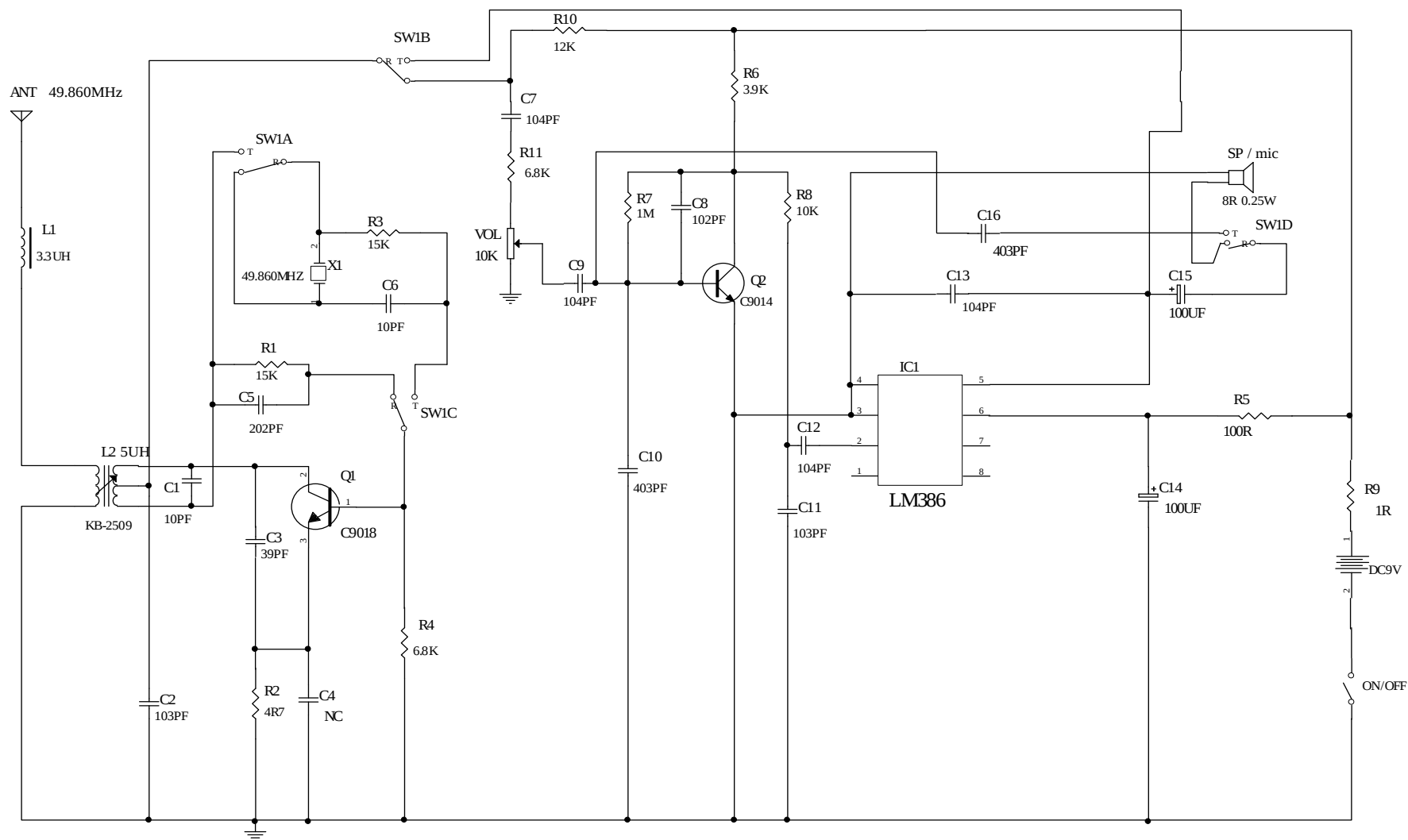
KS3159 SCHEMATIC
