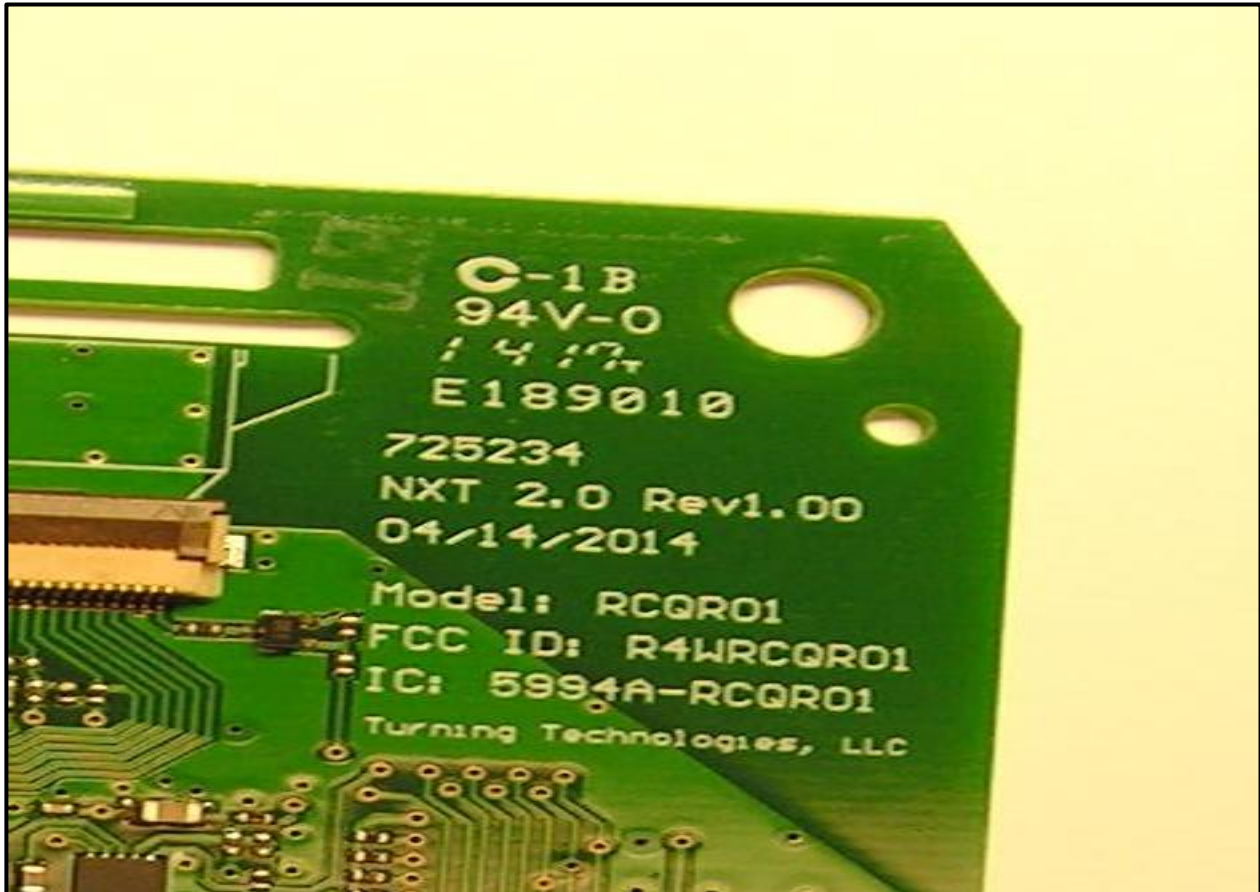
Photograph 1: ID Label on EUT
