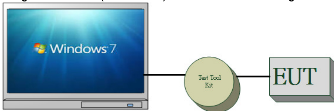
Fig. 2-1 Conducted (Antenna Port) & Radiated Emission Configuration
