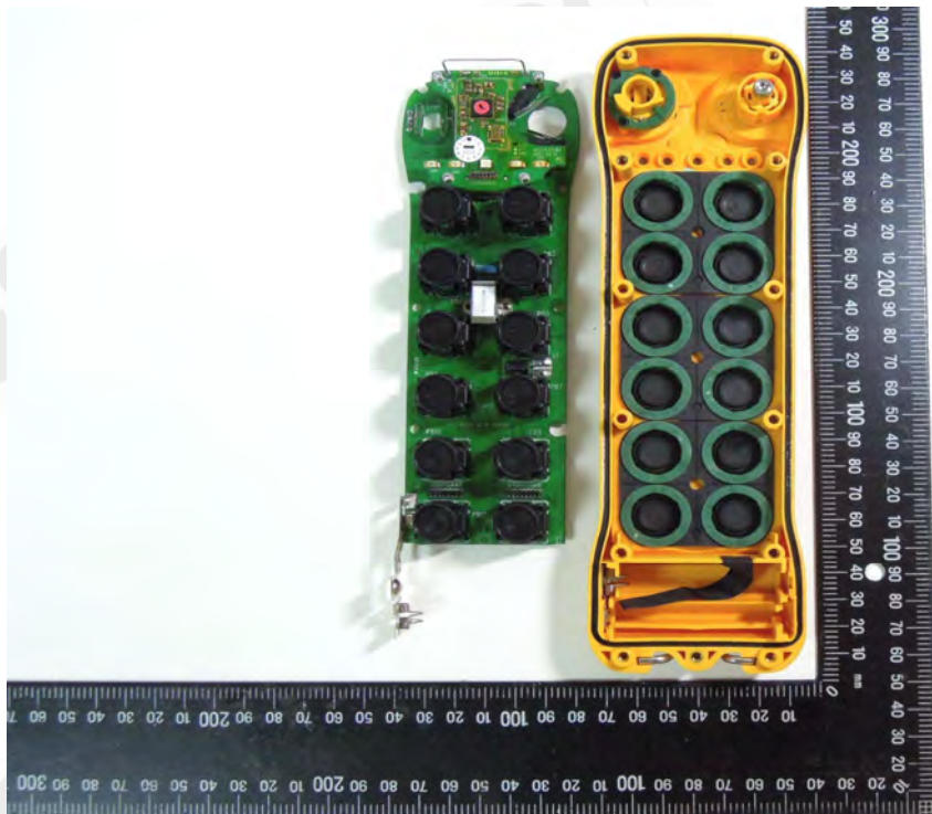
Internal View of EUT-1 (FLEX 12ES/12EX)
