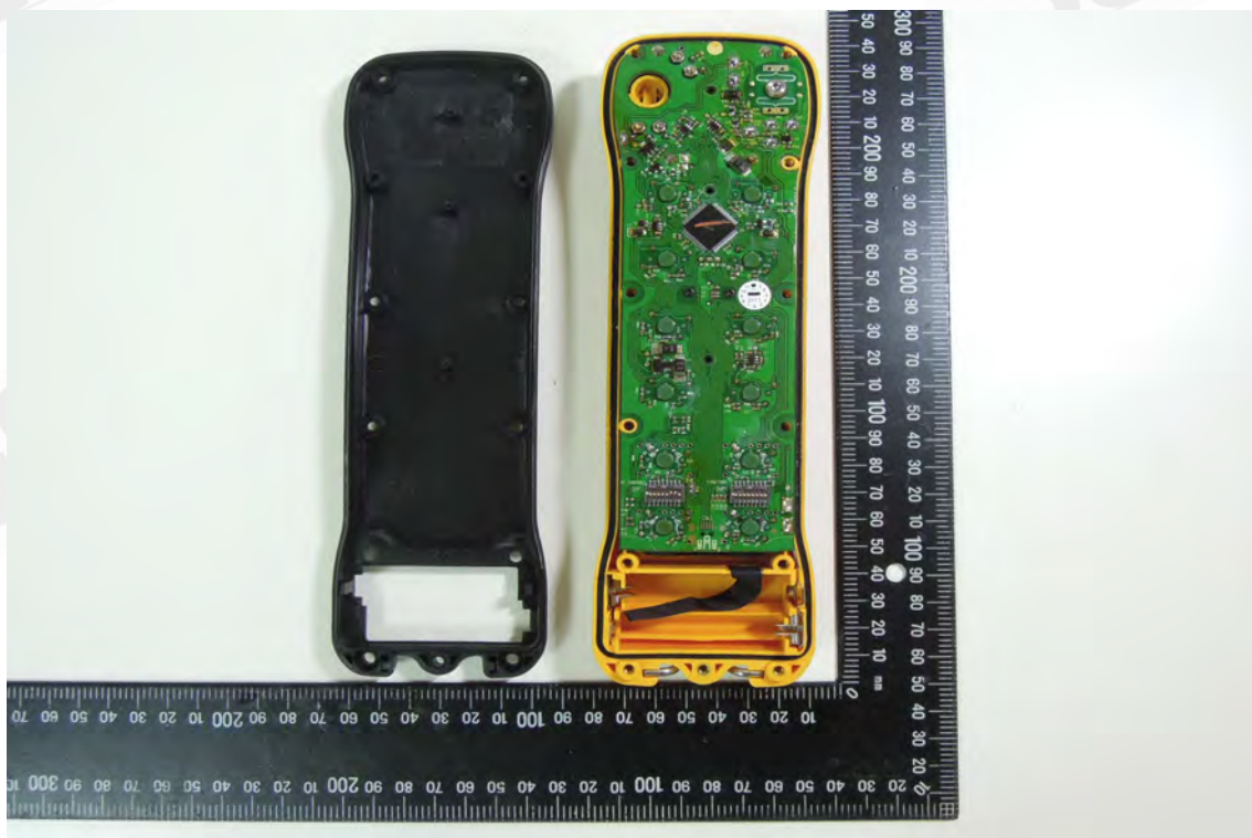
Open View of EUT-2 (FLEX 12ES/12EX)
