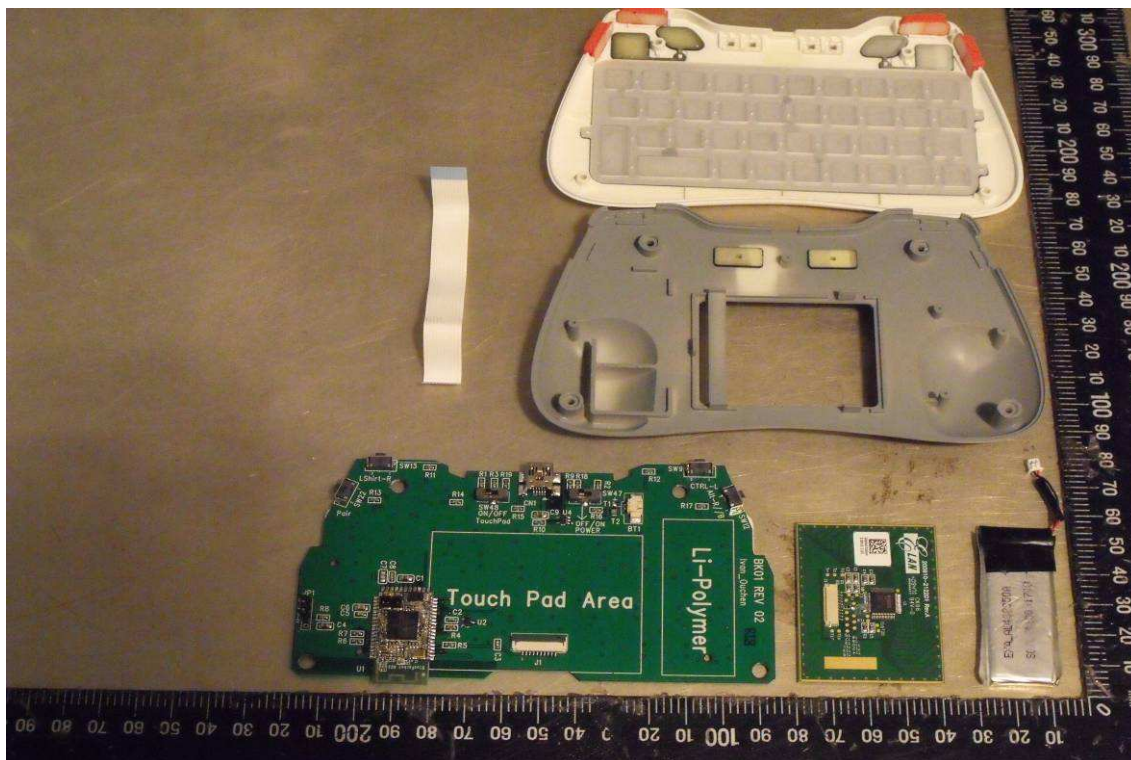
Inside View of Rear EUT-Rear
