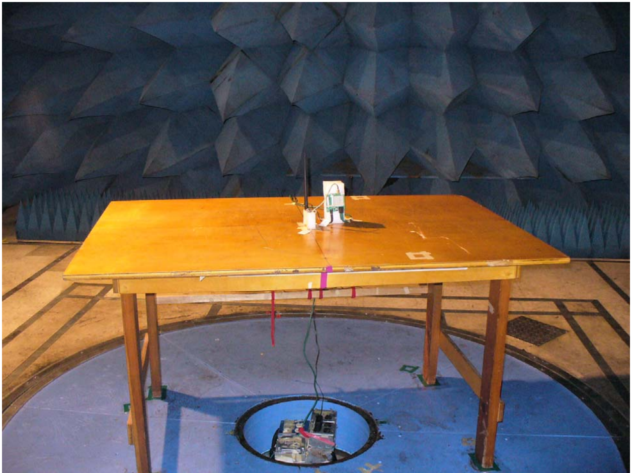
Figure 1: Radiated Emissions – EUT with Dipole Antenna (Front View)
