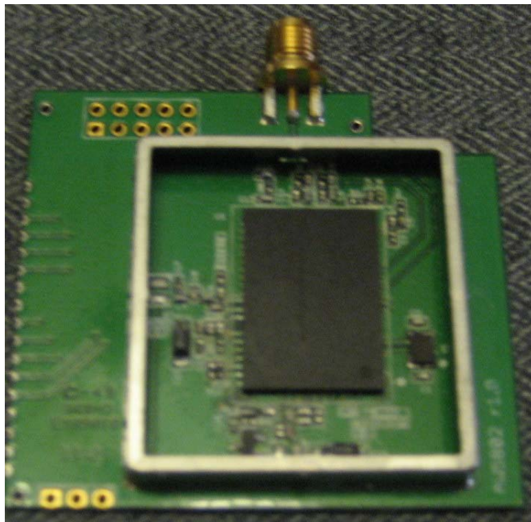
Figure 2 Top View (without shielding) – module standalone
