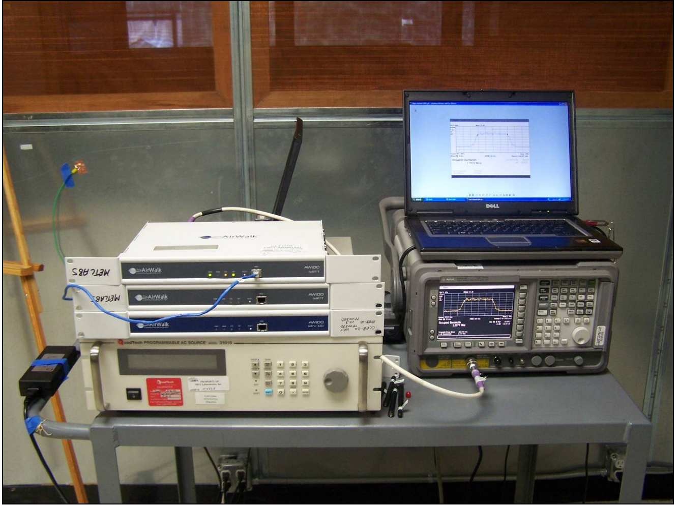
Photograph 3. Occupied Bandwidth, Test Setup
