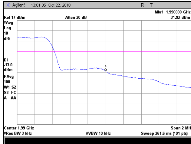
Plot 54. Frequency Stability, High Channel, High Voltage
