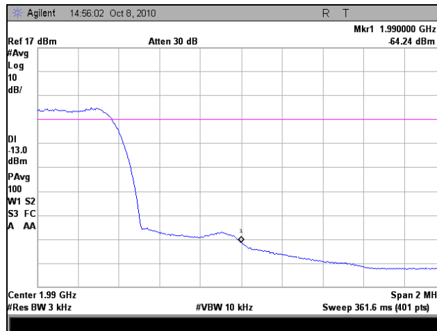
Plot 52. Frequency Stability, High Channel, 50°C
