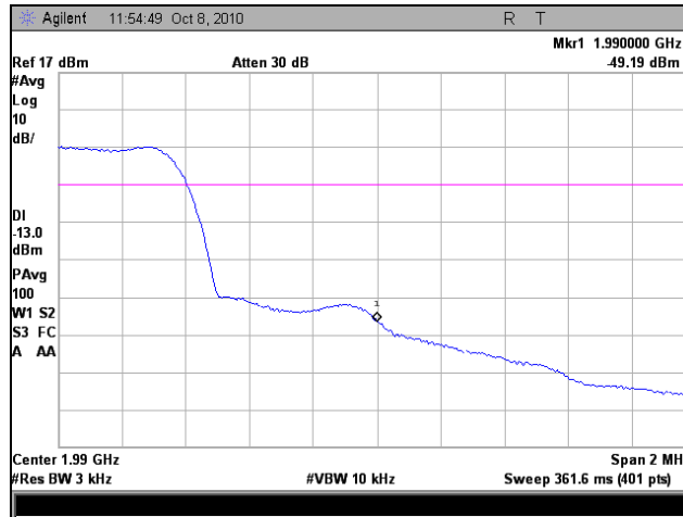
Plot 45. Frequency Stability, High Channel, -20°C
