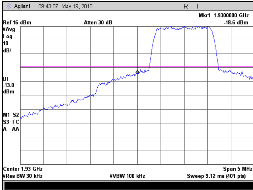
Plot 31. Band Edge, Low Channel
