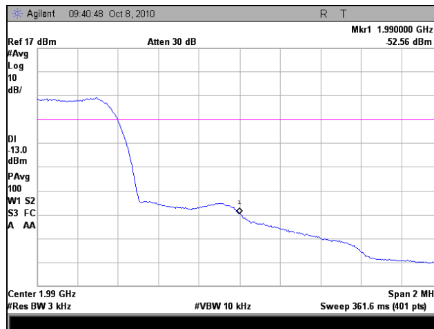
Plot 47. Frequency Stability, High Channel, 0°C
