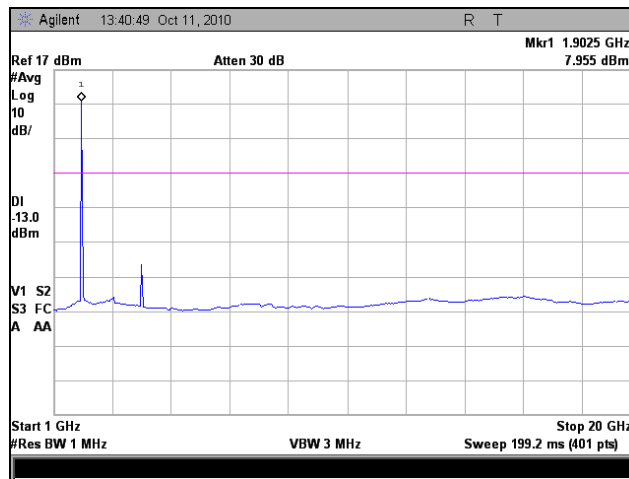
Plot 26. Conducted Spurious Emissions, Low Channel, 1 GHz – 20 GHz
