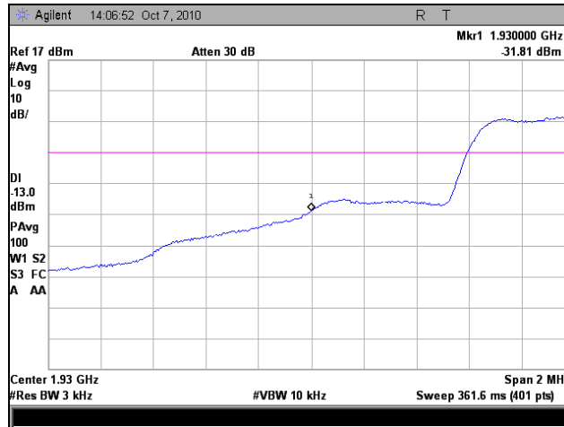
Plot 39. Frequency Stability, Low Channel, 30°C
