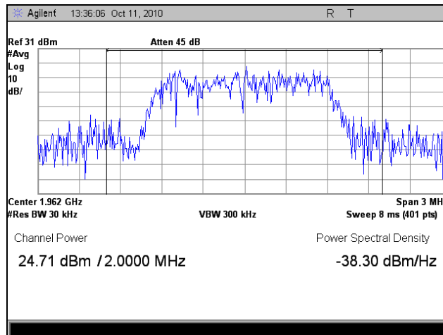
Plot 5. RF Power Output, Mid Channel, Average
