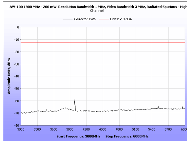
Plot 23. Radiated Spurious Emissions, High Channel, 3 GHz – 6 GHz
