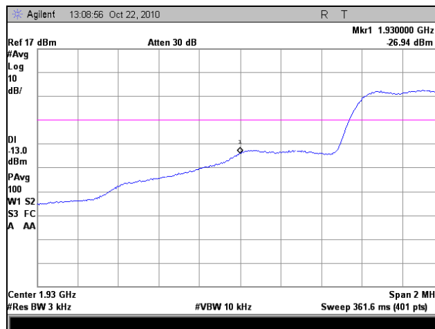
Plot 43. Frequency Stability, Low Channel, High Voltage
