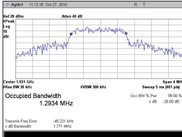
Plot 10. Occupied Bandwidth, Low Channel
