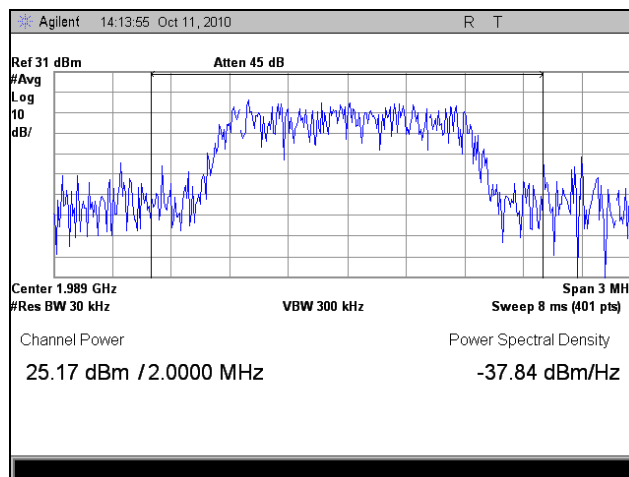
Plot 6. RF Power Output, High Channel, Average
