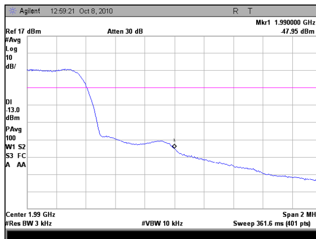
Plot 44. Frequency Stability, High Channel, -30°C
