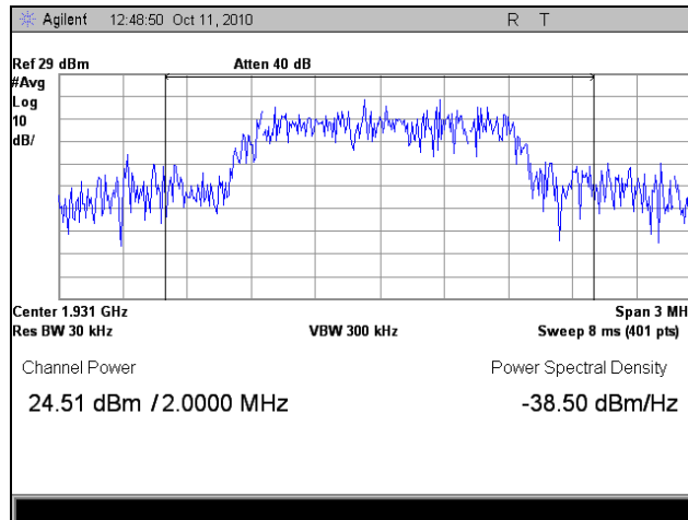
Plot 4. RF Power Output, Low Channel, Average
