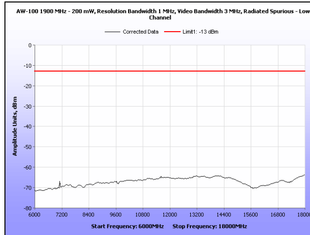
Plot 16. Radiated Spurious Emissions, Low Channel, 6 GHz – 18 GHz
