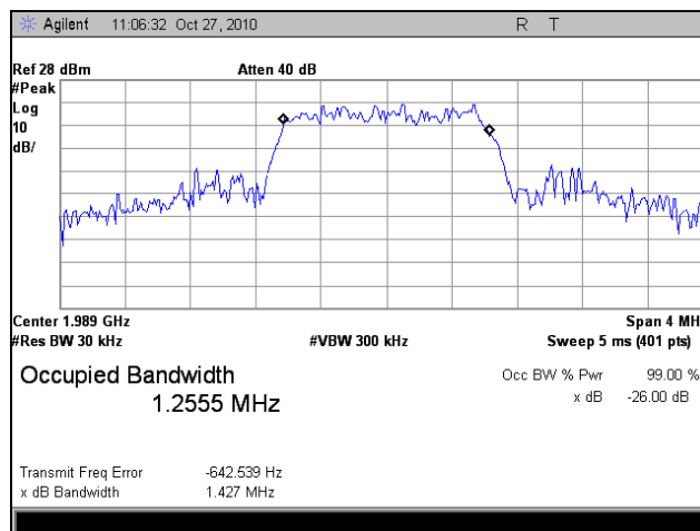
Plot 12. Occupied Bandwidth, High Channel
