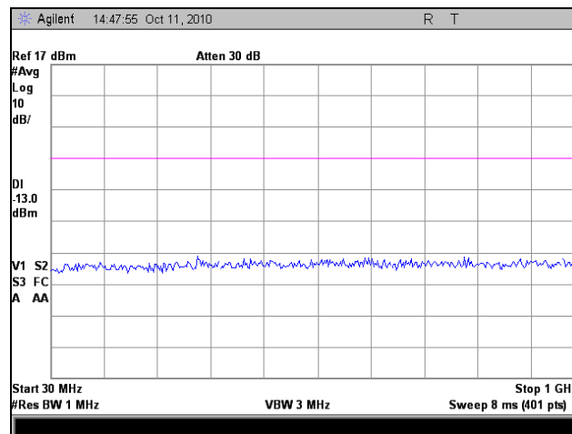
Plot 29. Conducted Spurious Emissions, High Channel, 30 MHz – 1 GHz
