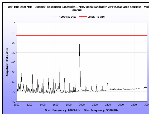
Plot 18. Radiated Spurious Emissions, Mid Channel, 1 GHz – 3 GHz
