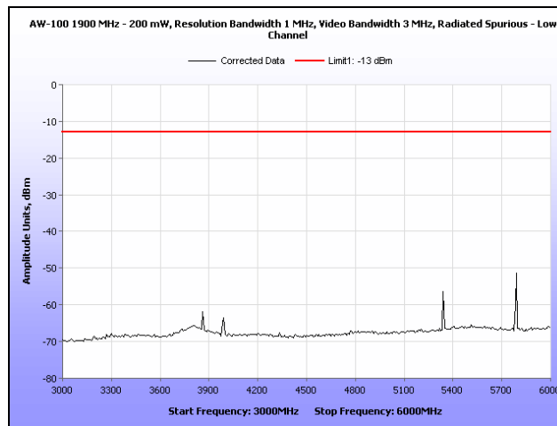
Plot 15. Radiated Spurious Emissions, Low Channel, 3 GHz – 6 GHz
