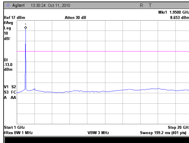
Plot 28. Conducted Spurious Emissions, Mid Channel, 1 GHz – 20 GHz
