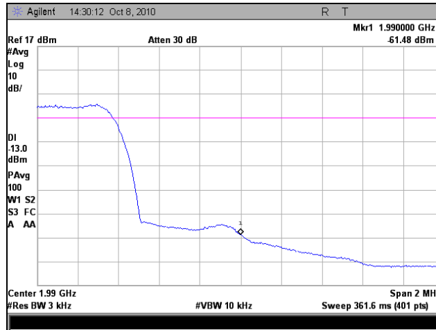
Plot 51. Frequency Stability, High Channel, 40°C
