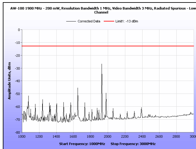
Plot 14. Radiated Spurious Emissions, Low Channel, 1 GHz – 3 GHz
