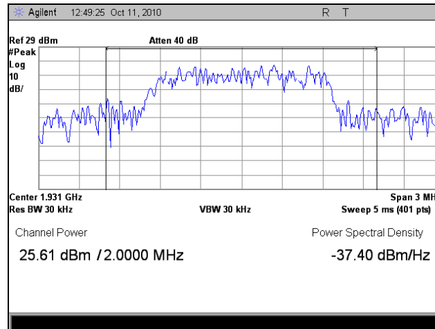
Plot 7. RF Power Output, Low Channel, Peak
