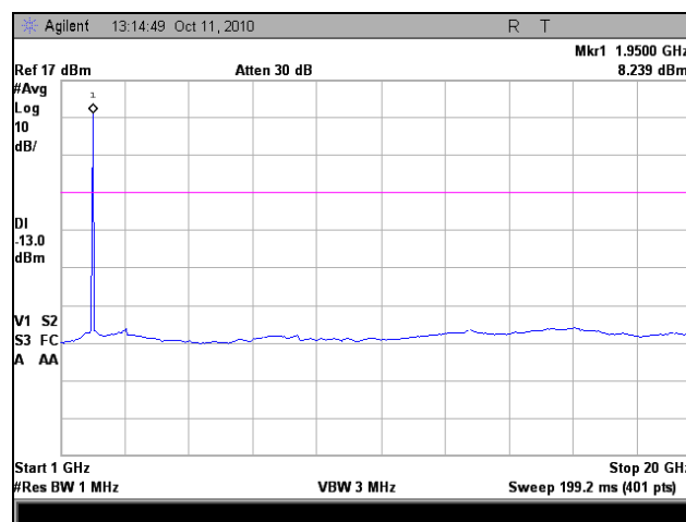
Plot 30. Conducted Spurious Emissions, High Channel, 1 GHz – 20 GHz
