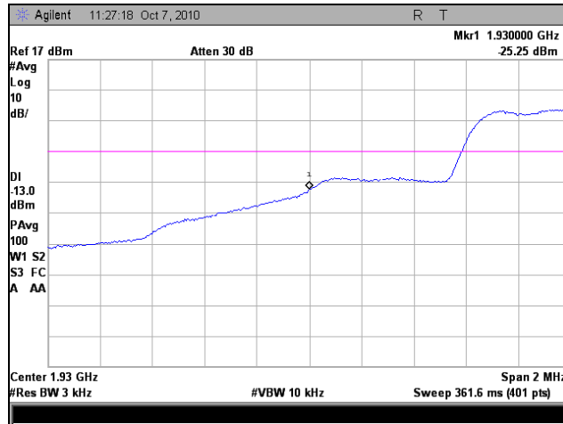
Plot 36. Frequency Stability, Low Channel, 0°C
