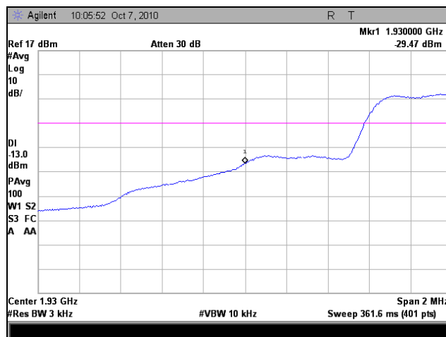
Plot 38. Frequency Stability, Low Channel, 20°C
