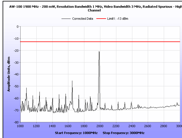
Plot 22. Radiated Spurious Emissions, High Channel, 1 GHz – 3 GHz
