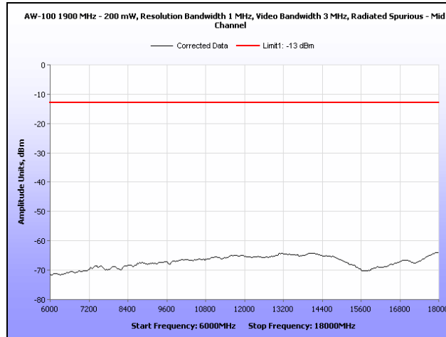
Plot 20. Radiated Spurious Emissions, Mid Channel, 6 GHz - 18 GHz
