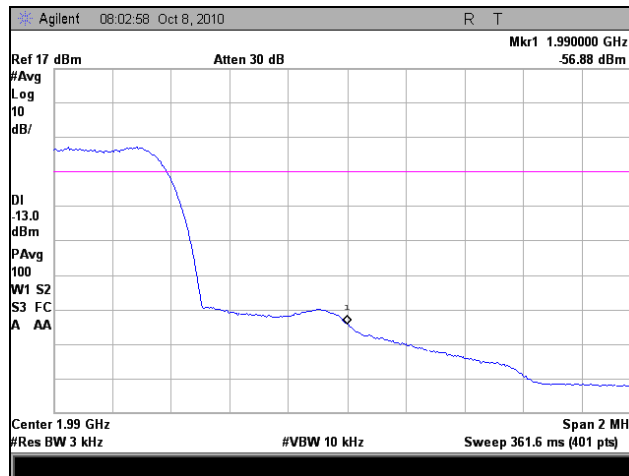
Plot 49. Frequency Stability, High Channel, 20°C
