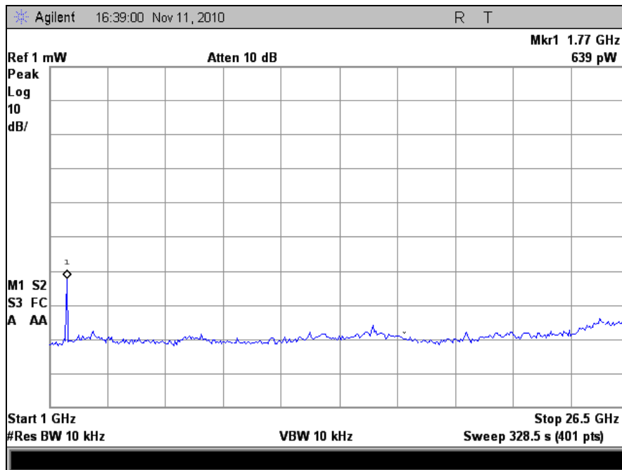
Plot 56. Receiver Spurious Emission, 1 GHz – 26.5 GHz
