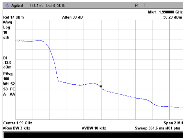
Plot 46. Frequency Stability, High Channel, -10°C
