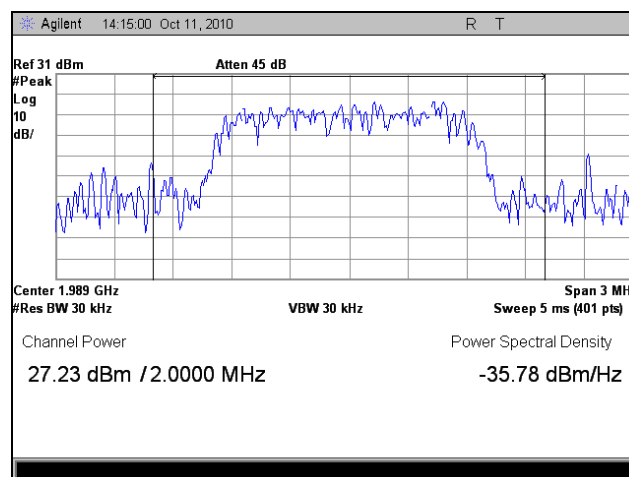
Plot 9. RF Power Output, High Channel, Peak
