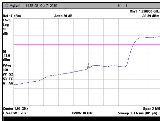
Plot 41. Frequency Stability, Low Channel, 50°C
