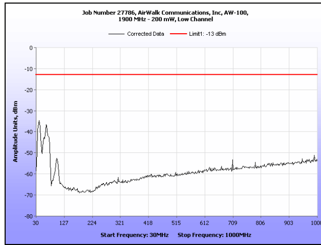
Plot 13. Radiated Spurious Emissions, Low Channel, 30 MHz – 1 GHz
