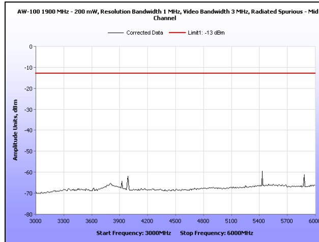
Plot 19. Radiated Spurious Emissions, Mid Channel, 3 GHz - 6 GHz
