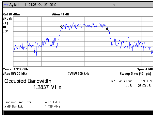
Plot 11. Occupied Bandwidth, Mid Channel
