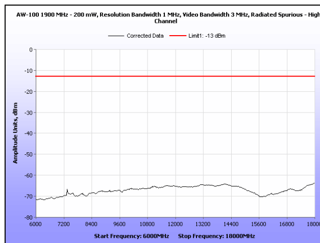
Plot 24. Radiated Spurious Emissions, High Channel, 6 GHz – 18 GHz
