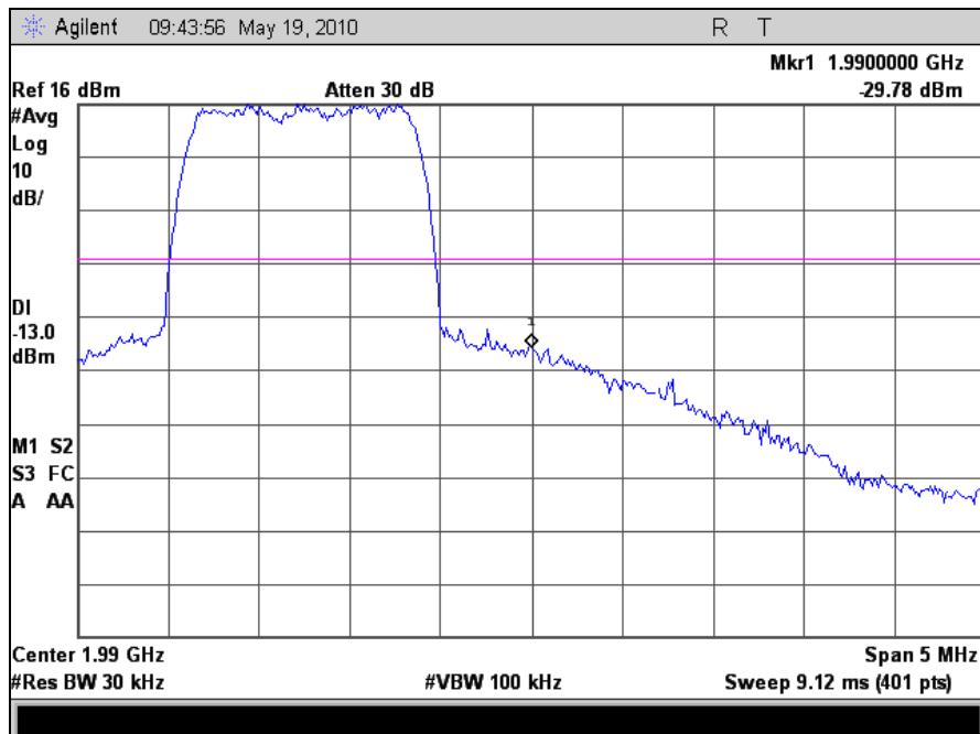
Plot 32. Band Edge, High Channel
