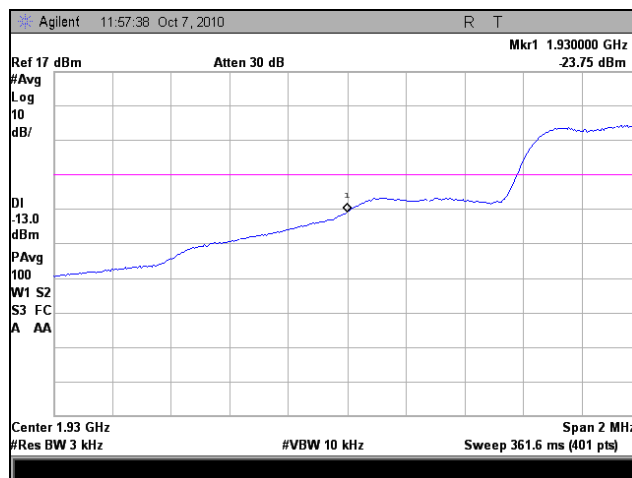
Plot 35. Frequency Stability, Low Channel, -10°C
