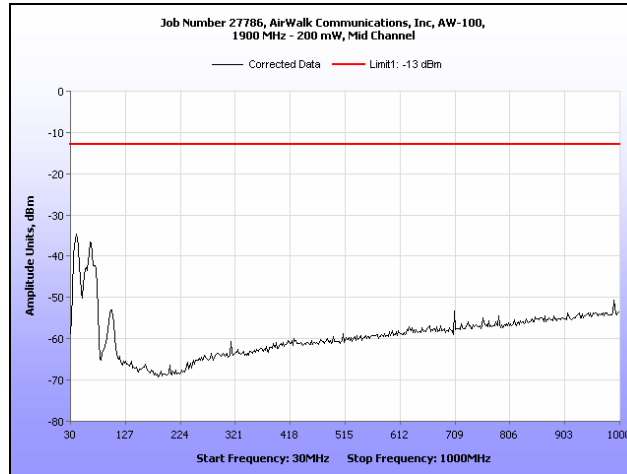
Plot 17. Radiated Spurious Emissions, Mid Channel, 30 MHz – 1 GHz
