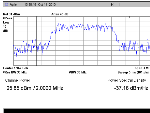
Plot 8. RF Power Output, Mid Channel, Peak
