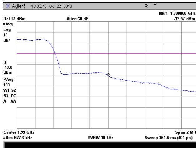
Plot 53. Frequency Stability, High Channel, Low Voltage
