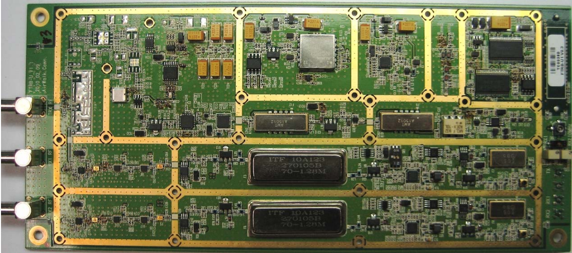
Photograph 6. FTRB-U1 Top
