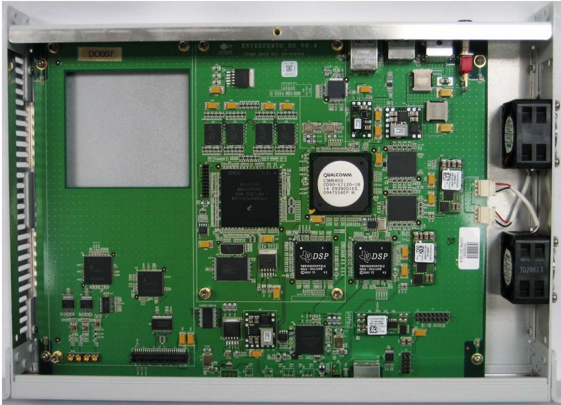
Photograph 3. AW100 800MHz 200mW - Digital Board
