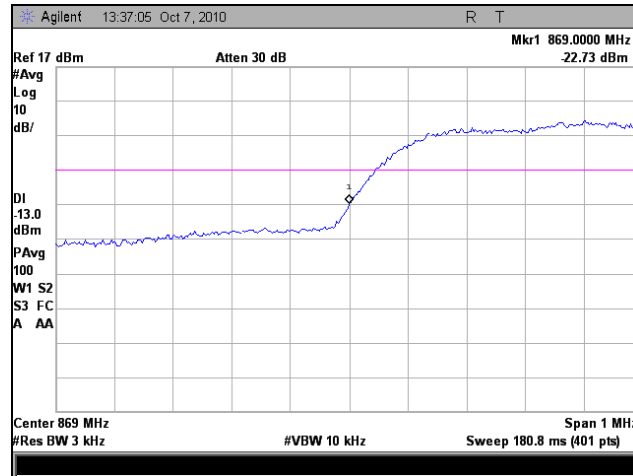
Plot 35. Frequency Stability, Low Channel, -30°C
