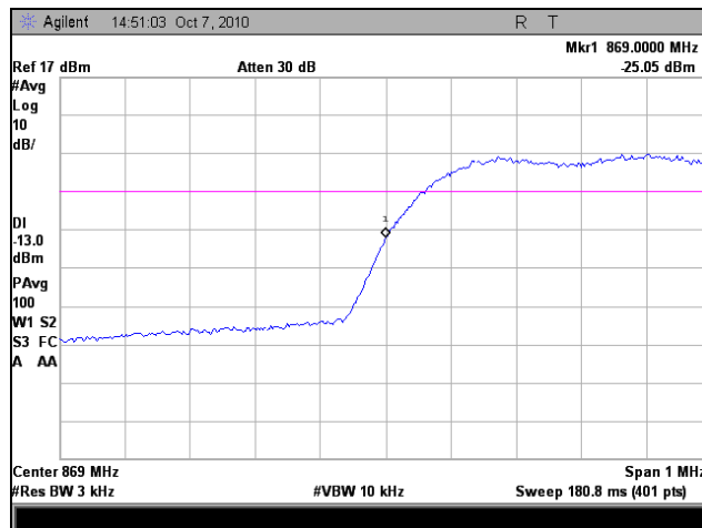
Plot 43. Frequency Stability, Low Channel, 50°C
