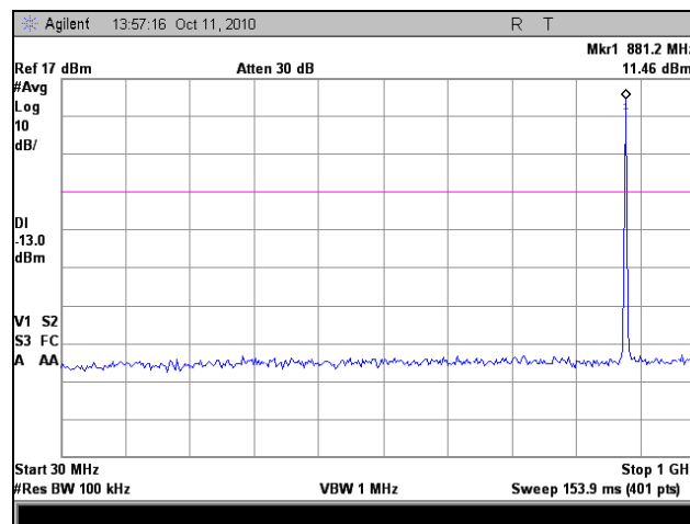
Plot 29. Conducted Spurious Emissions, Mid Channel, 30 MHz – 1 GHz
