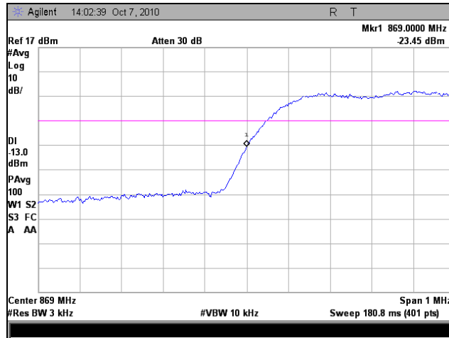
Plot 41. Frequency Stability, Low Channel, 30°C
