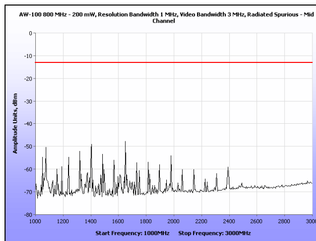
Plot 20. Radiated Spurious Emissions, Mid Channel, 1 GHz – 3 GHz
