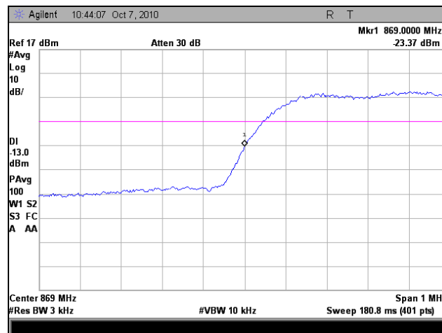
Plot 39. Frequency Stability, Low Channel, 10°C
