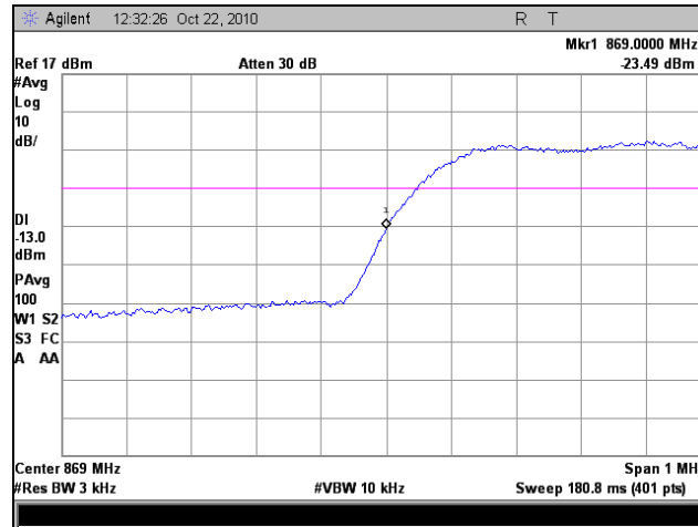
Plot 44. Frequency Stability, Low Channel, Low Voltage
