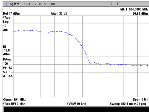
Plot 56. Frequency Stability, High Channel, High Voltage
