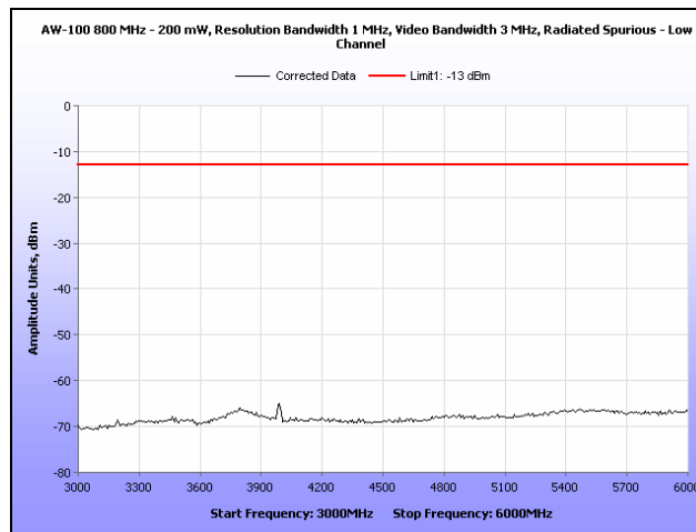
Plot 17. Radiated Spurious Emissions, Low Channel, 3 GHz – 6 GHz
