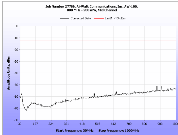
Plot 19. Radiated Spurious Emissions, Mid Channel, 30 MHz – 1 GHz
