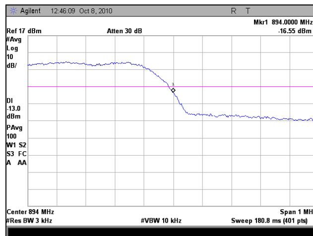
Plot 46. Frequency Stability, High Channel, -30°C
