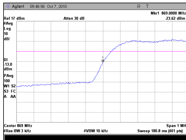
Plot 40. Frequency Stability, Low Channel, 20°C
