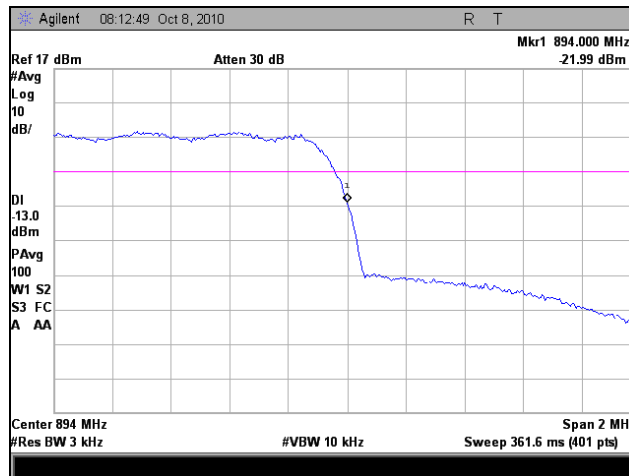
Plot 51. Frequency Stability, High Channel, 20°C
