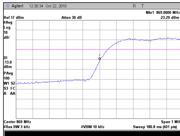
Plot 45. Frequency Stability, Low Channel, High Voltage
