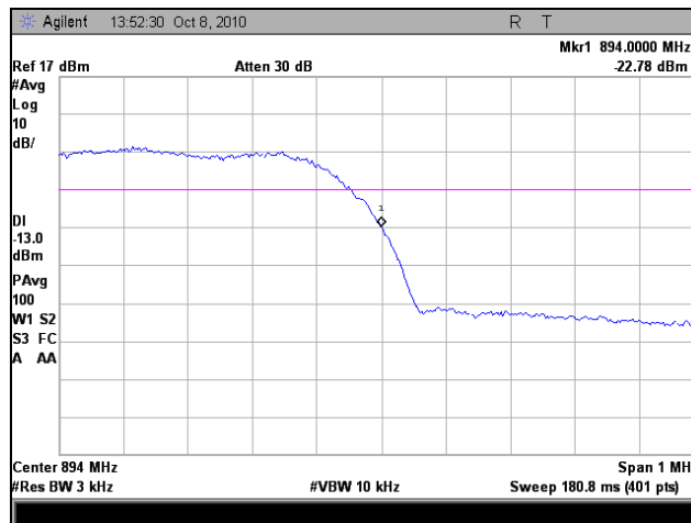
Plot 52. Frequency Stability, High Channel, 30°C
