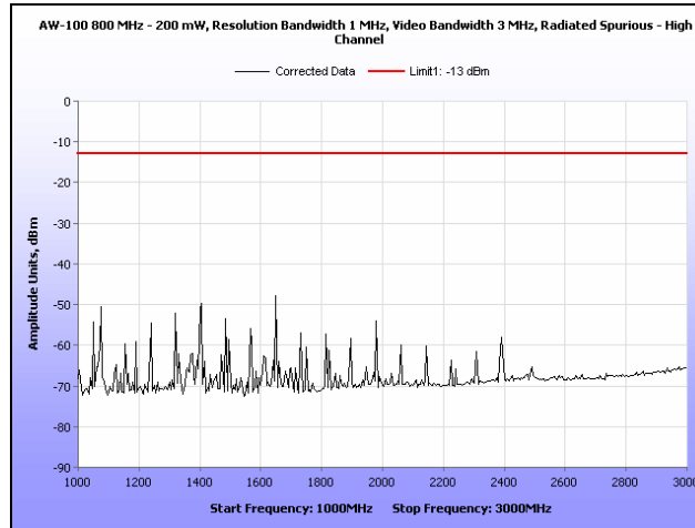
Plot 24. Radiated Spurious Emissions, High Channel, 1 GHz – 3 GHz
