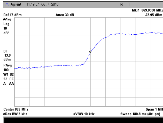
Plot 38. Frequency Stability, Low Channel, 0°C
