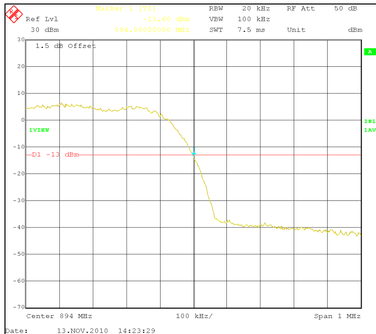
Plot 34. Band Edge, High Channel
