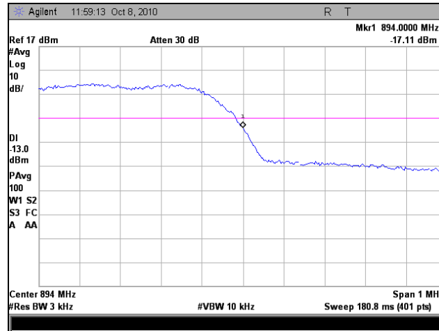
Plot 47. Frequency Stability, High Channel, -20°C
