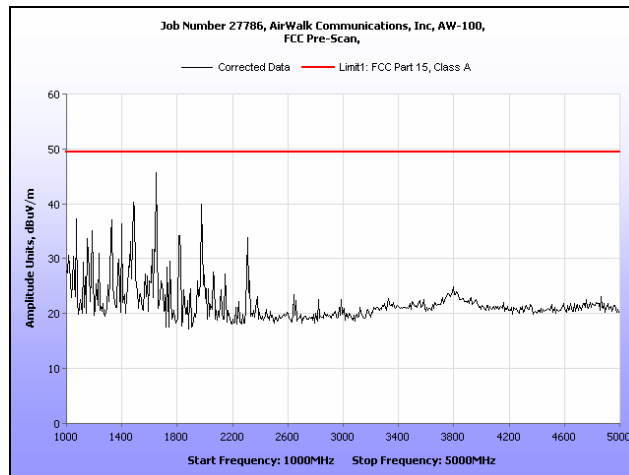
Plot 5. Radiated Emissions, Pre-Scan, 1 GHz – 5 GHz, Peak
