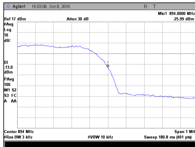
Plot 54. Frequency Stability, High Channel, 50°C
