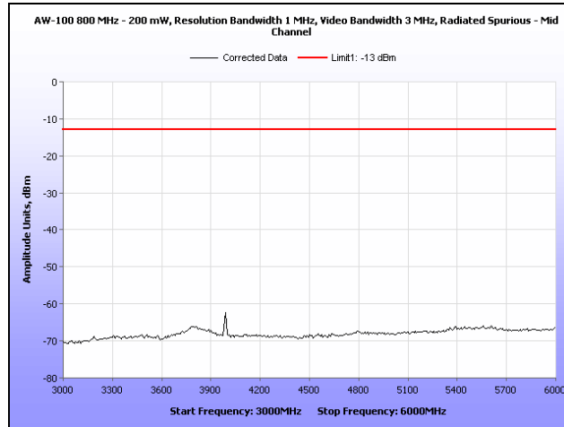
Plot 21. Radiated Spurious Emissions, Mid Channel, 3 GHz - 6 GHz
