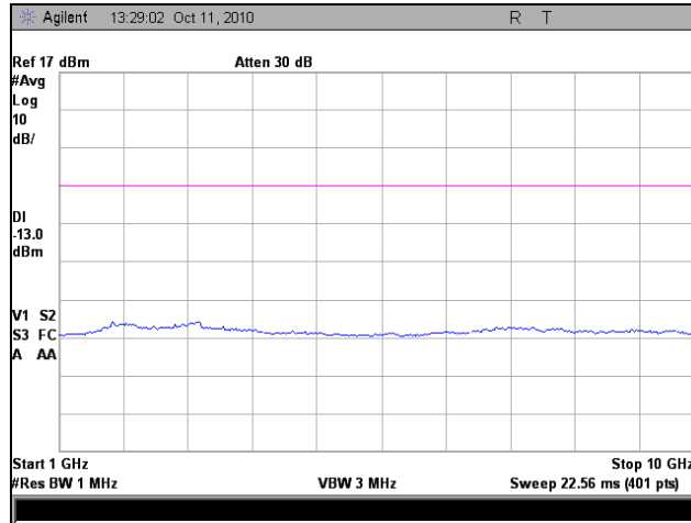
Plot 30. Conducted Spurious Emissions, Mid Channel, 1 GHz – 10 GHz
