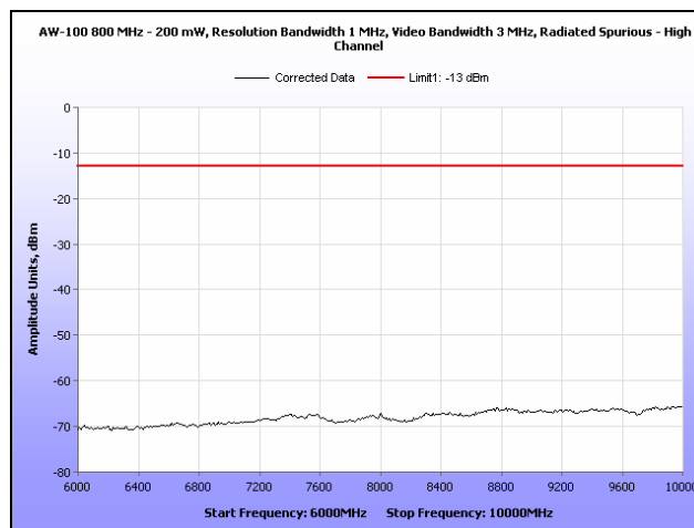
Plot 26. Radiated Spurious Emissions, High Channel, 6 GHz – 10 GHz
