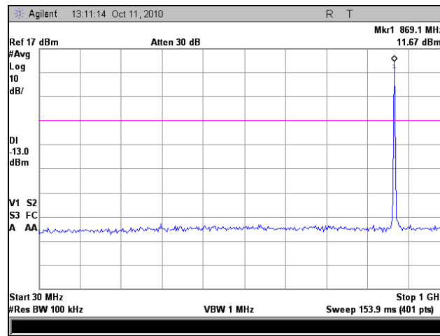
Plot 27. Conducted Spurious Emissions, Low Channel, 30 MHz – 1 GHz
