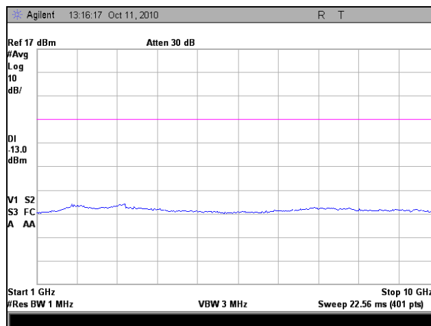
Plot 32. Conducted Spurious Emissions, High Channel, 1 GHz – 10 GHz
