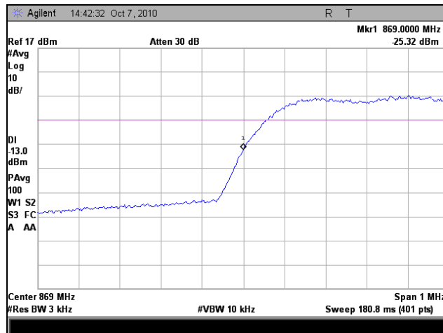
Plot 42. Frequency Stability, Low Channel, 40°C
