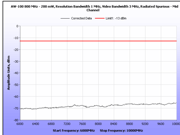
Plot 22. Radiated Spurious Emissions, Mid Channel, 6 GHz - 10 GHz
