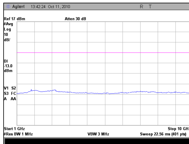
Plot 28. Conducted Spurious Emissions, Low Channel, 1 GHz – 10 GHz
