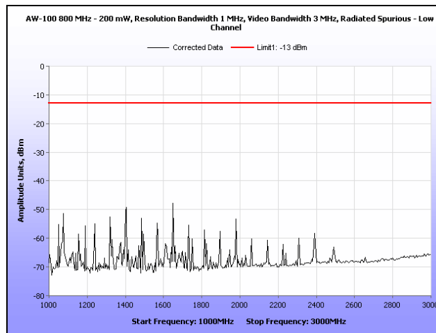
Plot 16. Radiated Spurious Emissions, Low Channel, 1 GHz – 3 GHz
