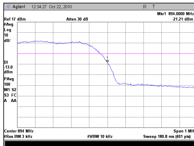
Plot 55. Frequency Stability, High Channel, Low Voltage
