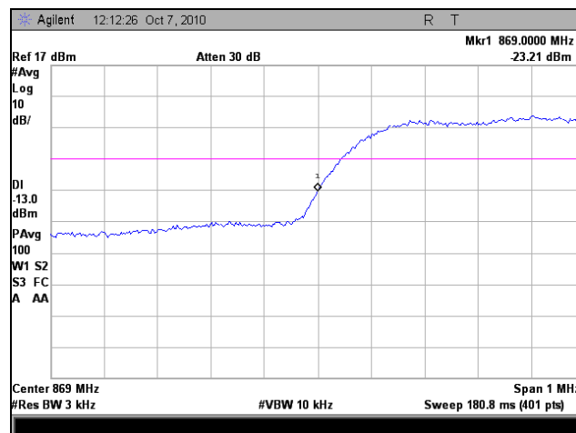
Plot 37. Frequency Stability, Low Channel, -10°C
