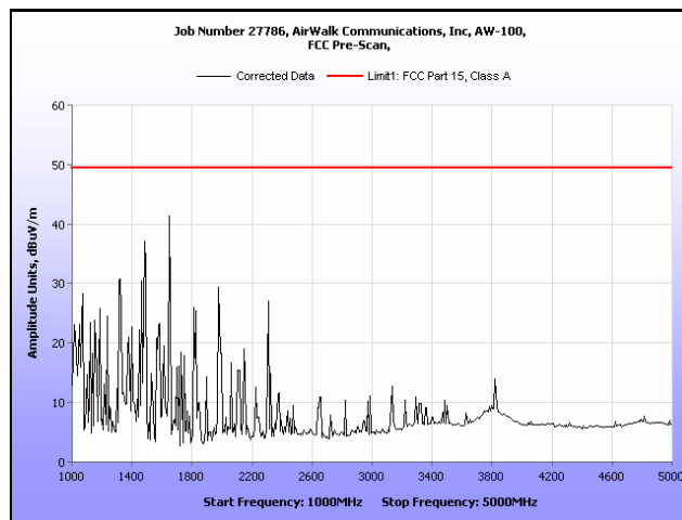
Plot 4. Radiated Emissions, Pre-Scan, 1 GHz – 5 GHz, Average
