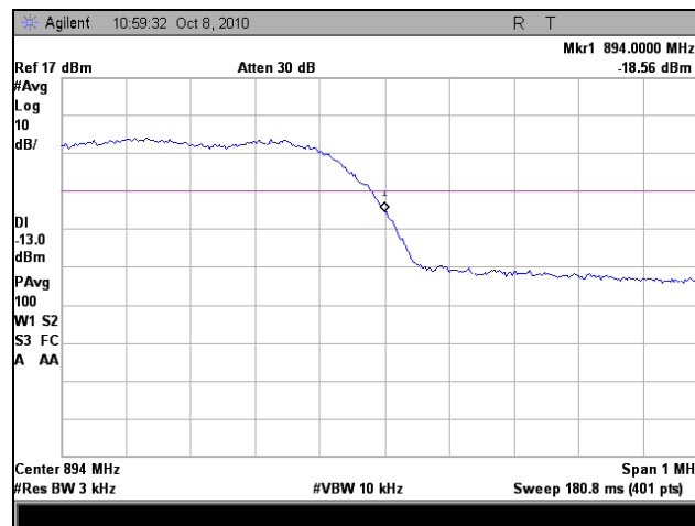
Plot 48. Frequency Stability, High Channel, -10°C
