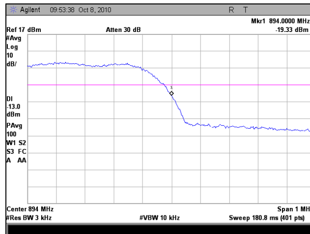
Plot 49. Frequency Stability, High Channel, 0°C
