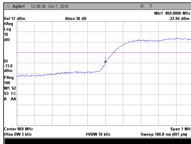
Plot 36. Frequency Stability, Low Channel, -20°C
