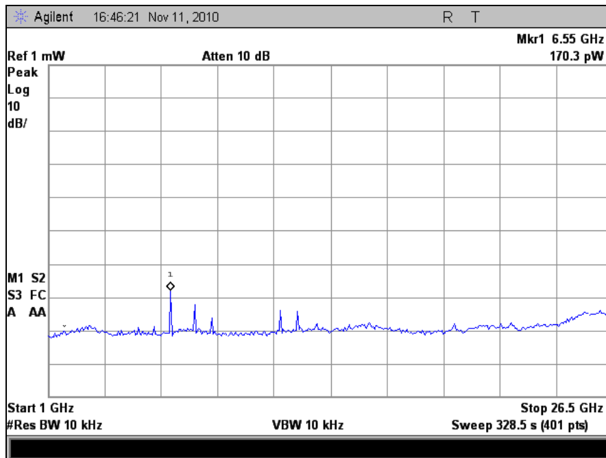
Plot 58. Receiver Spurious Emission, 1 GHz – 26.5 GHz
