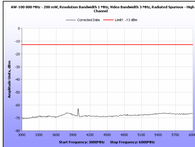
Plot 25. Radiated Spurious Emissions, High Channel, 3 GHz – 6 GHz
