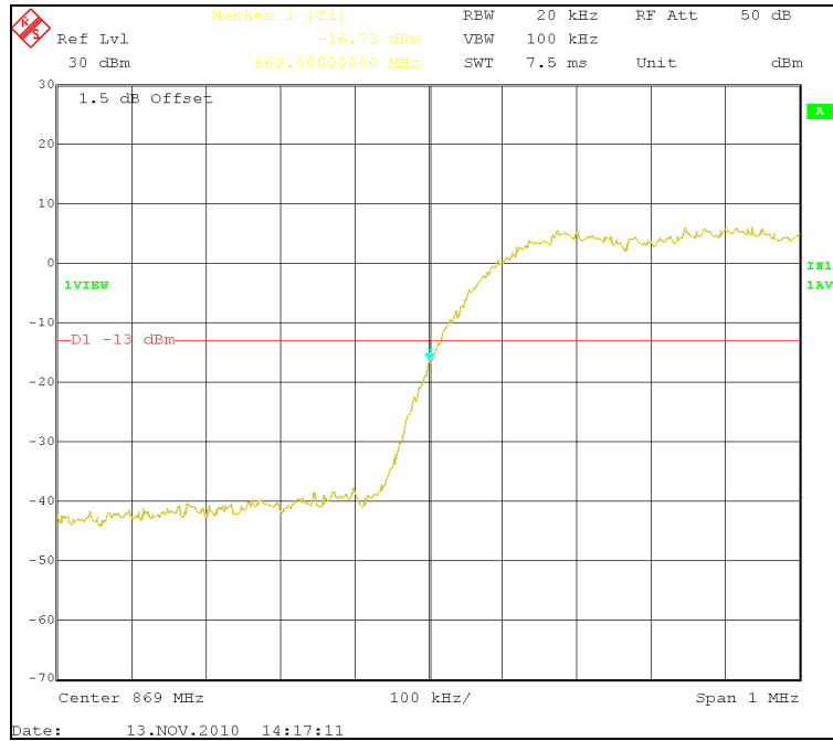
Plot 33. Band Edge, Low Channel
