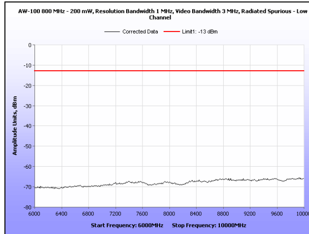
Plot 18. Radiated Spurious Emissions, Low Channel, 6 GHz – 10 GHz
