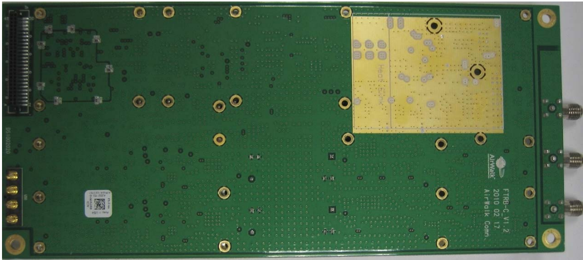
Photograph 4. FTRB-C1 Bottom
