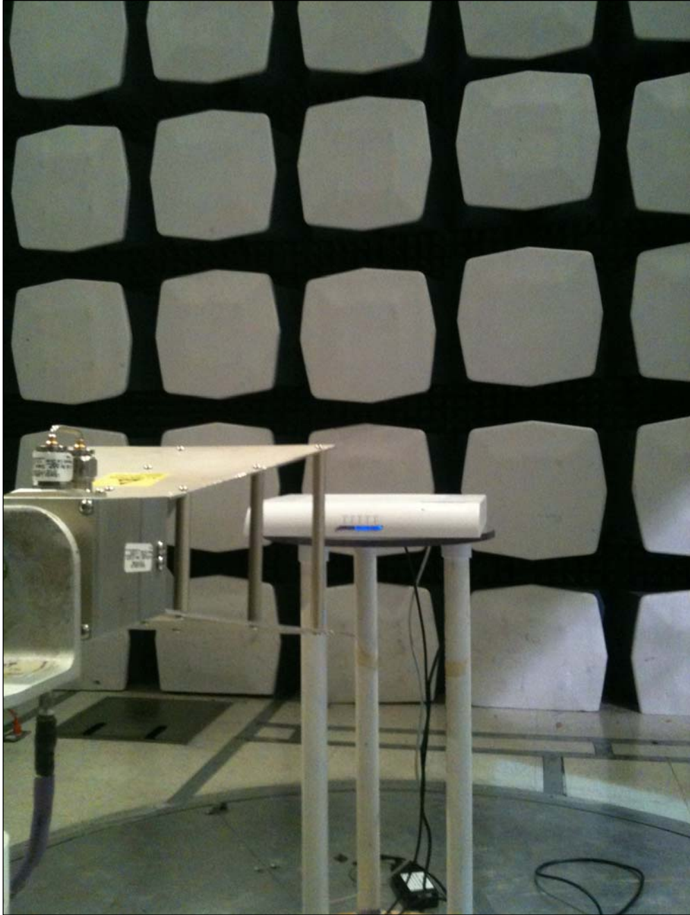
Photograph 4. Radiated Spurious, Test Setup
