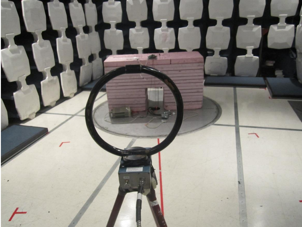
Radiated Emissions – 9 KHz to 30 MHz
