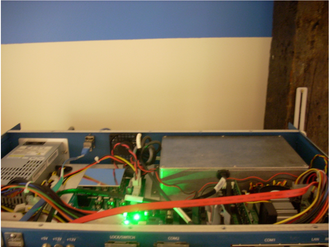
The RF module is inside the aluminum box on the right side Please see next page for top view
