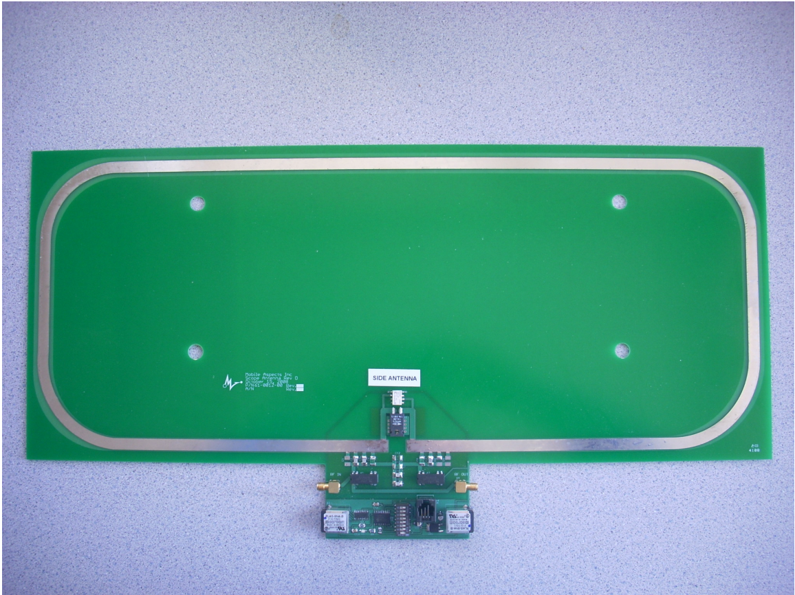
Side - Antenna
