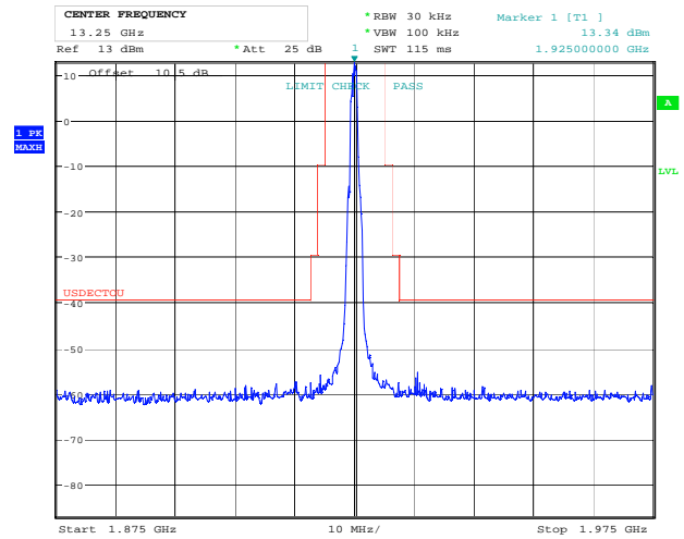
Out-of-Band Emissions, Middle Channel
