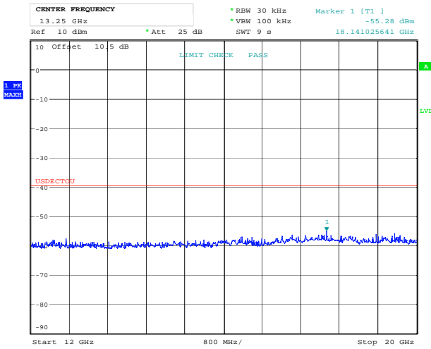
Out-of-Band Emissions, Middle Channel
