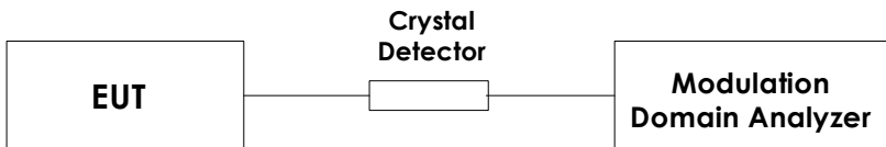
Test Set-up 2
