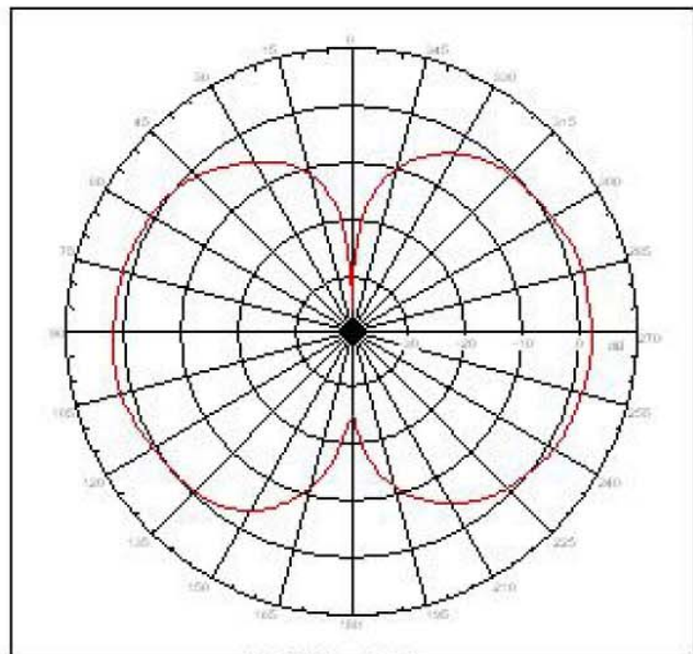
2.45GHz_E-plane
