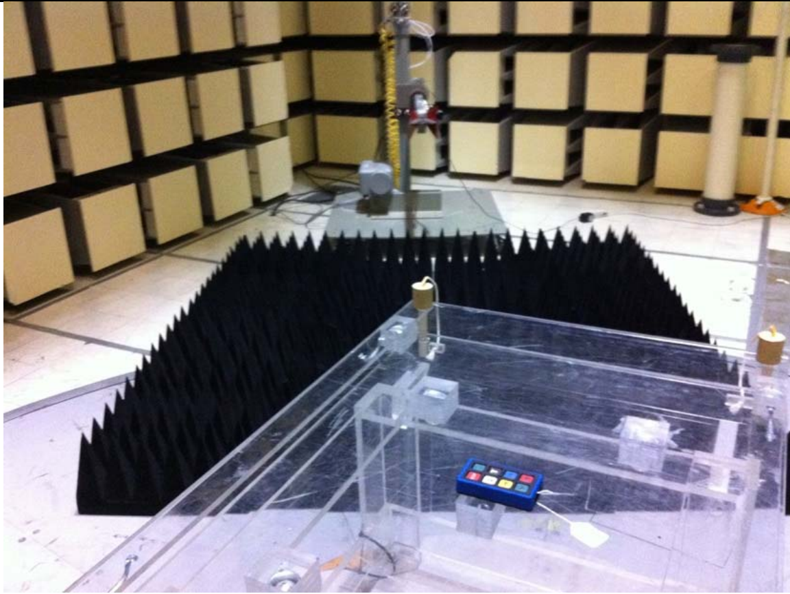
Radiated Tests 1 to 18 GHz
