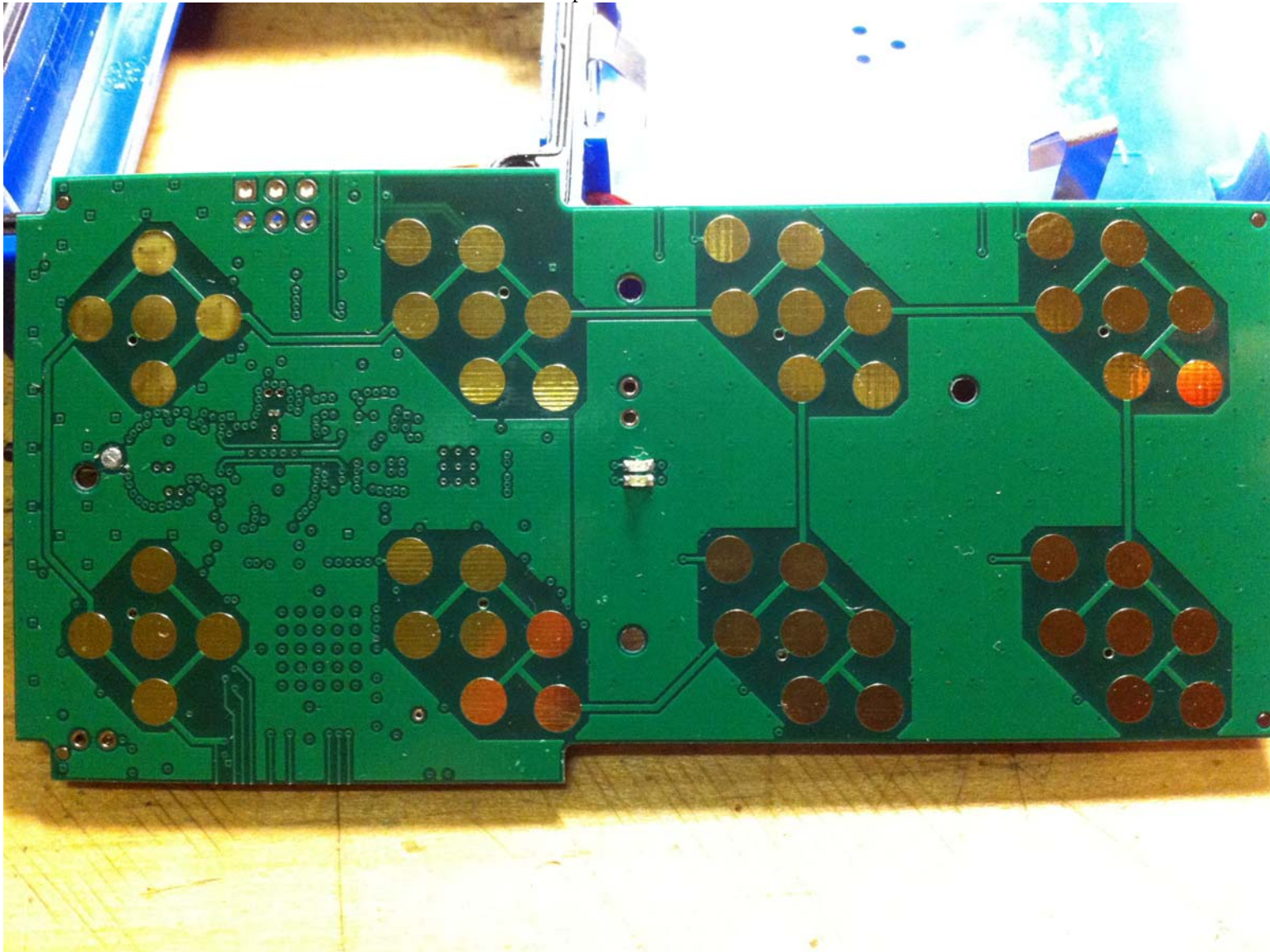
Figure 3 Overall View of Circuit Board Assembly - Bottom or Keyboard Side
