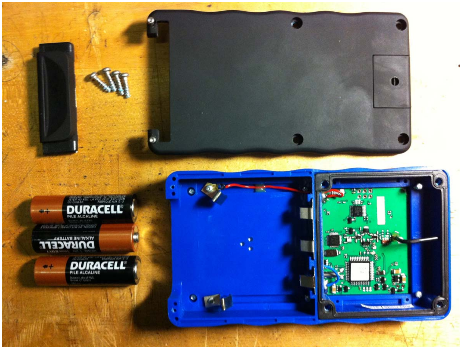
Figure 1 Bottom Cover Removed - View of Interior
