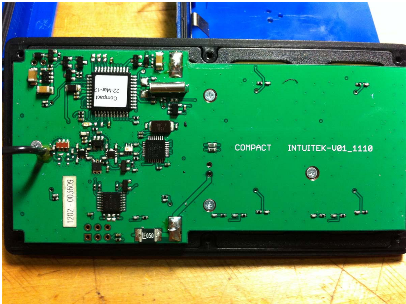
Figure 2 Overall View of Circuit Board Assembly - Top
