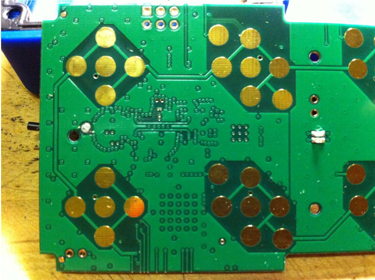
Figure 5 Close Up View of Component Placement on PCA - Bottom
