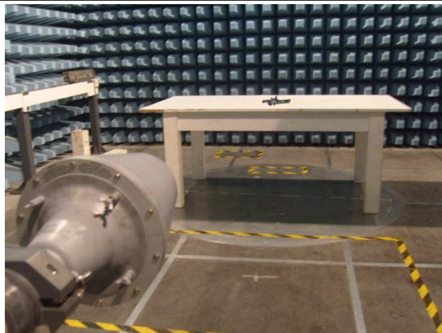
PHOTO 2 – RADIATED EMISSION SETUP
