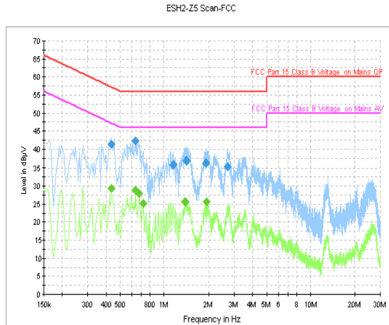
Fig. 33 AC Power line Conducted Emission (Traffic, AE3)
