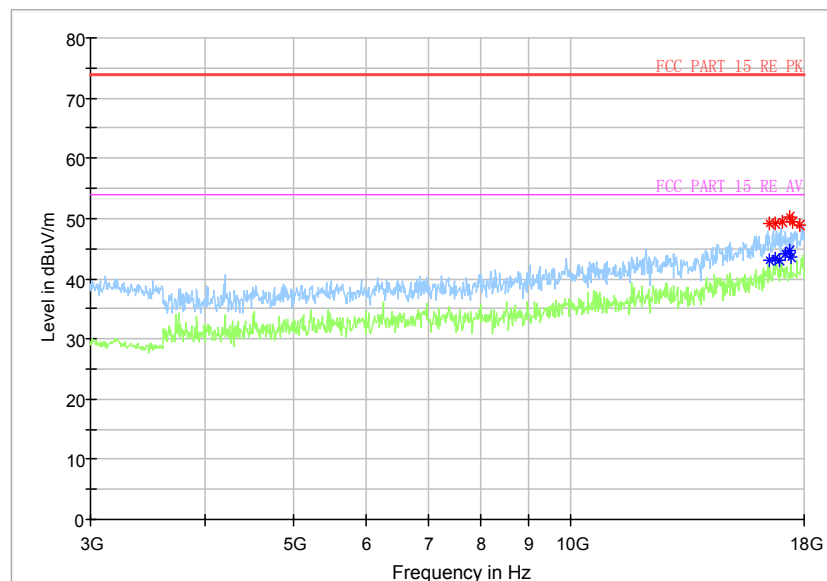
BT_2DH5_CH39
