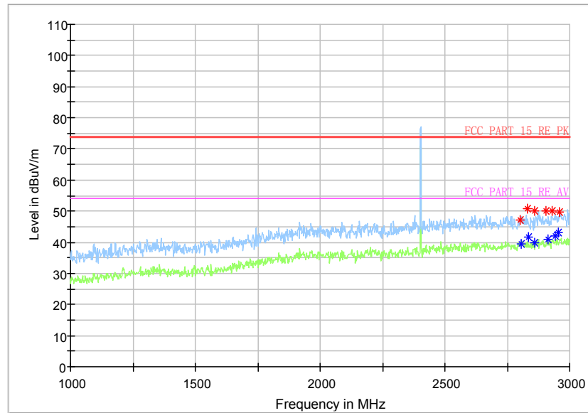
BT_2DH5_CH0
