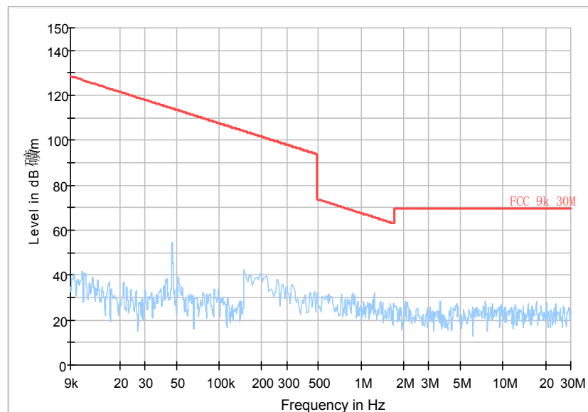
BT_3DH5_CH39
