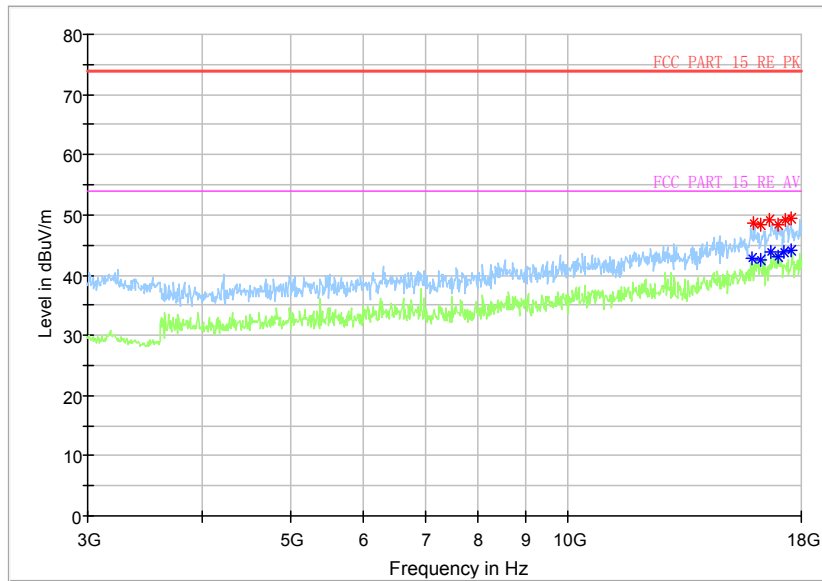
BT_2DH5_CH78
