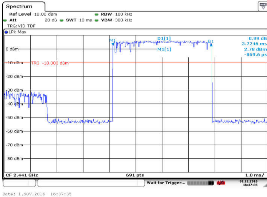
Fig. 92 Time of Occupancy(Dwell Time) (GFSK, Ch39)
