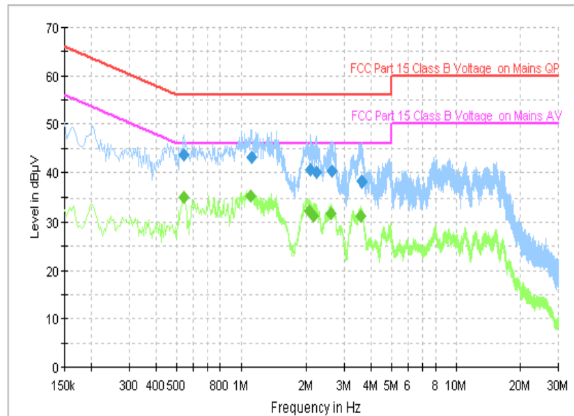
Fig. 108 AC Power line Conducted Emission (Idle, AE1)
