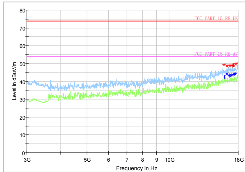
BT_DH5_CH39
