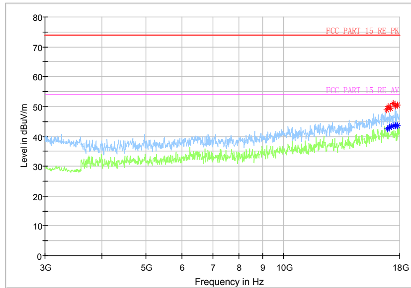
BT_3DH5_CH0
