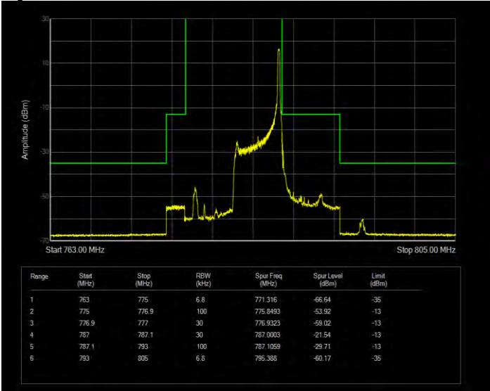
Band13 QPSK BW=5MHz Channel=23255 RB Size=25 Position=#0 Extended
