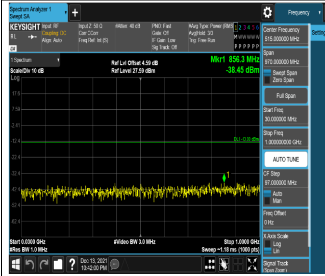
Band2-1.4MHz-16QAM-18607-1RB#0-Range1:30~1000MHz
