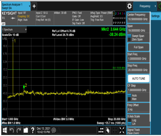
Band2-1.4MHz-16QAM-18607-1RB#0-Range2:1000~20000MHz
