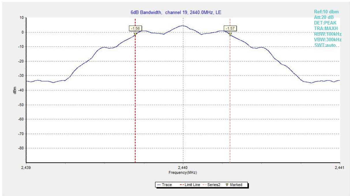
Fig.17 6dB Bandwidth (Ch 19), LE Coded
