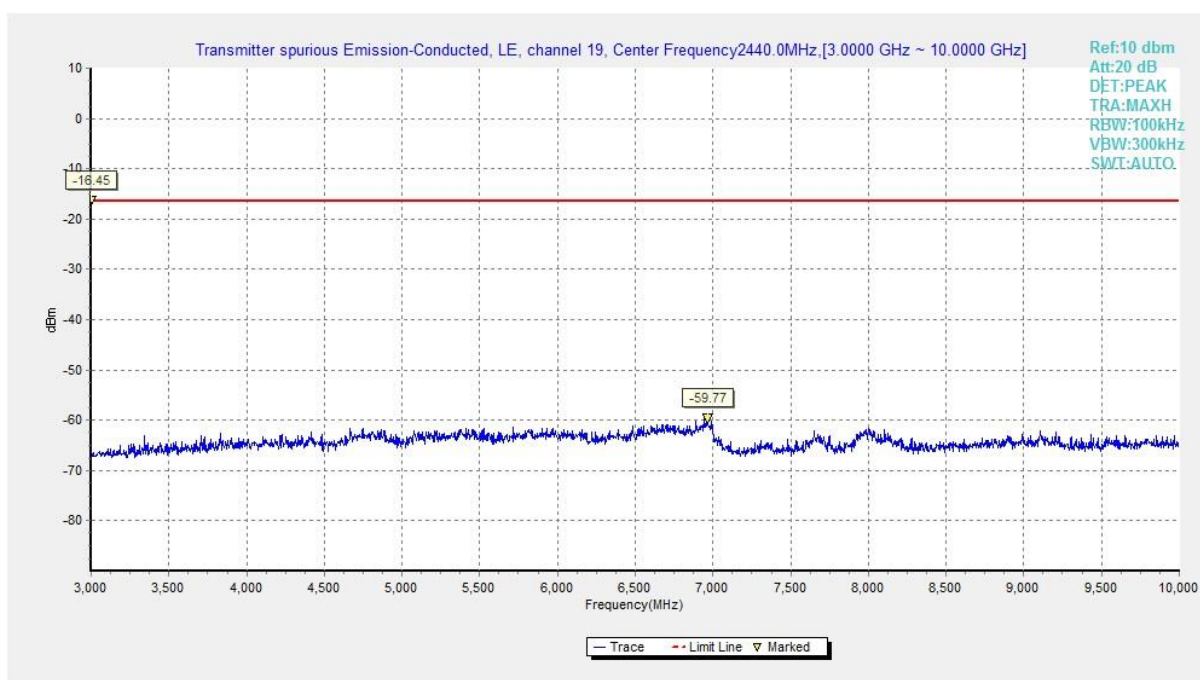
Fig.30 Conducted Spurious Emission (Ch19, 3 GHz-10 GHz), LE 1M
