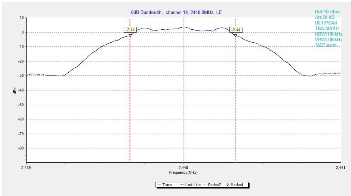
Fig.11 6dB Bandwidth (Ch 19), LE 1M
