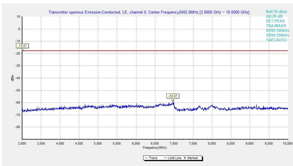
Fig.38 Conducted Spurious Emission (Ch0, 3 GHz-10 GHz), LE 2M
