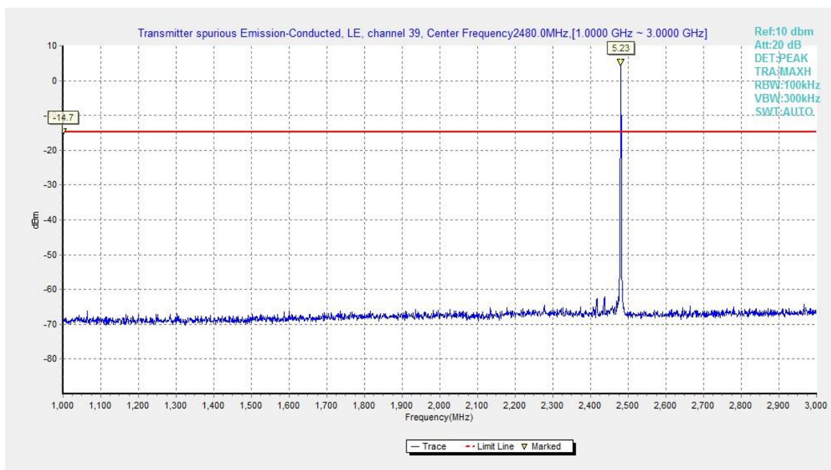
Fig.43 Conducted Spurious Emission (Ch39, 1 GHz-3 GHz), LE 2M
