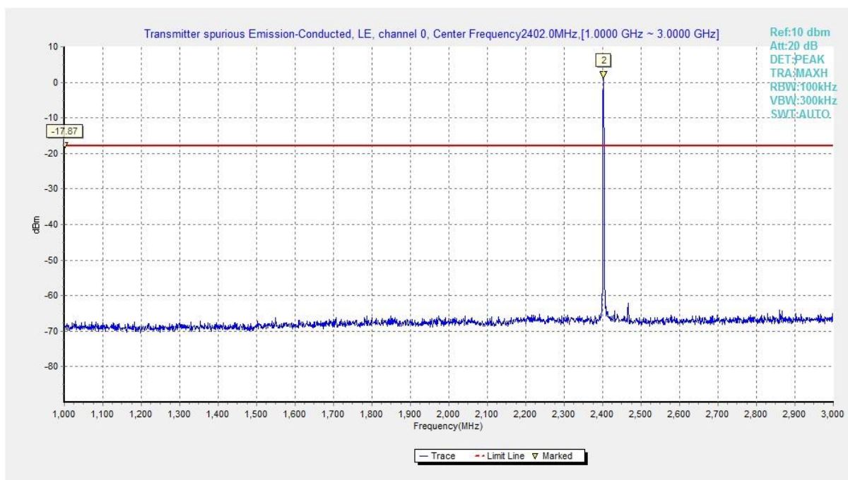
Fig.37 Conducted Spurious Emission (Ch0, 1 GHz-3 GHz), LE 2M
