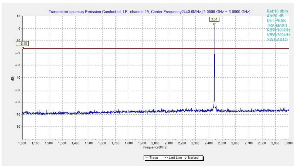
Fig.29 Conducted Spurious Emission (Ch19, 1 GHz-3 GHz), LE 1M
