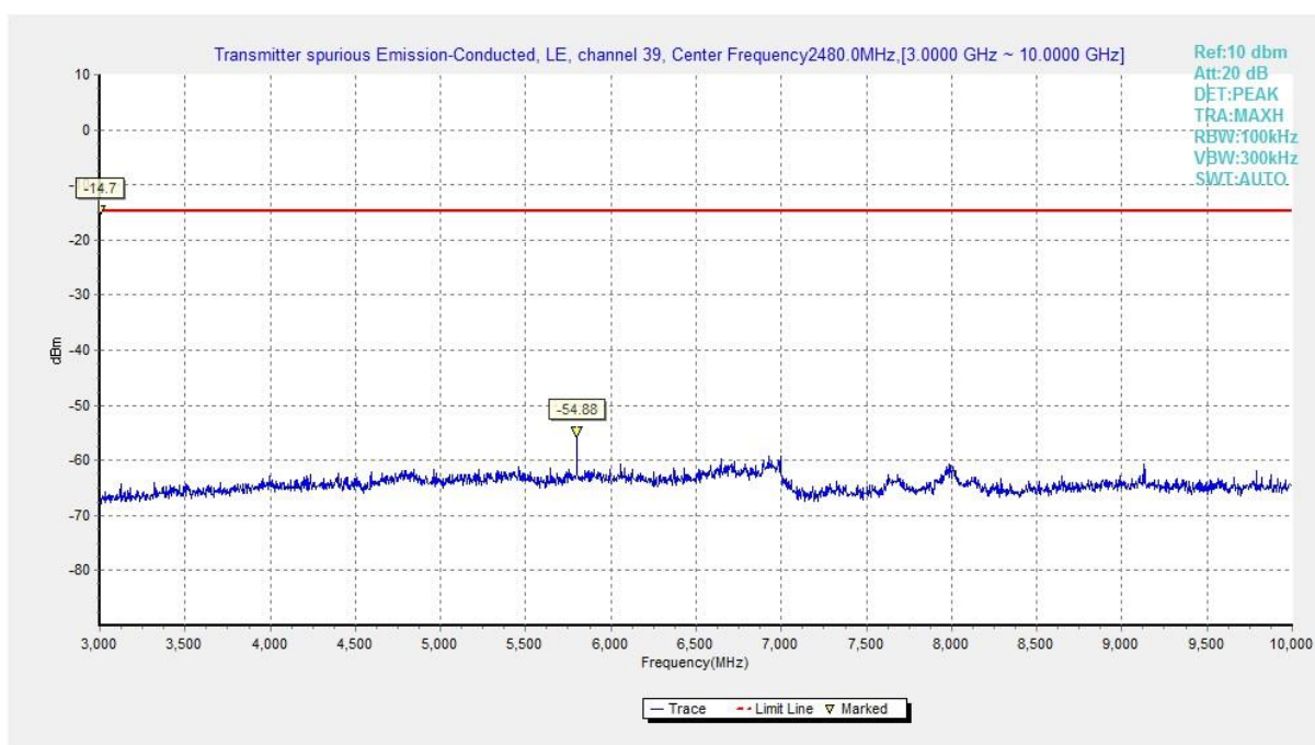
Fig.44 Conducted Spurious Emission (Ch39, 3 GHz-10 GHz), LE 2M
