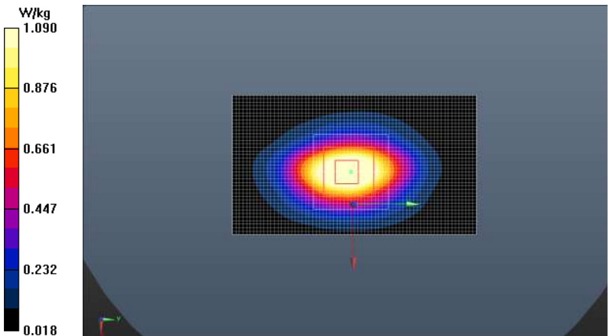
Fig.20 LTE Band 4
