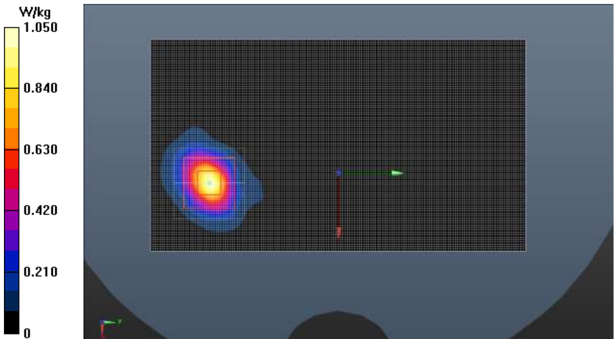
Fig.42 WLAN 5G
