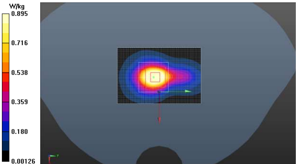
Fig.34 LTE Band 41
