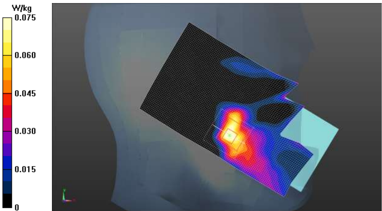
Fig.33 LTE Band 41
