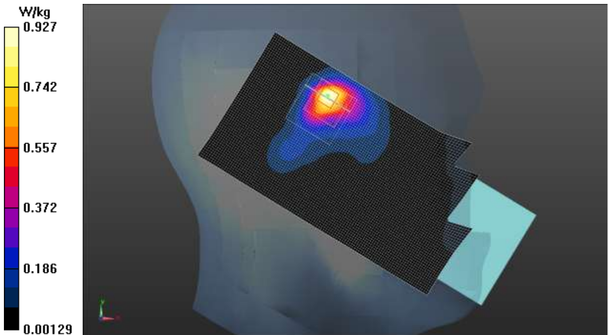
Fig.39 WLAN 2.4G
