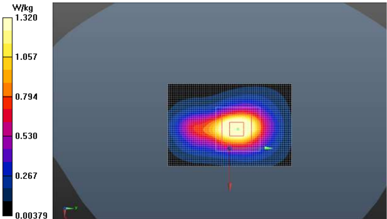
Fig.24 LTE Band 7
