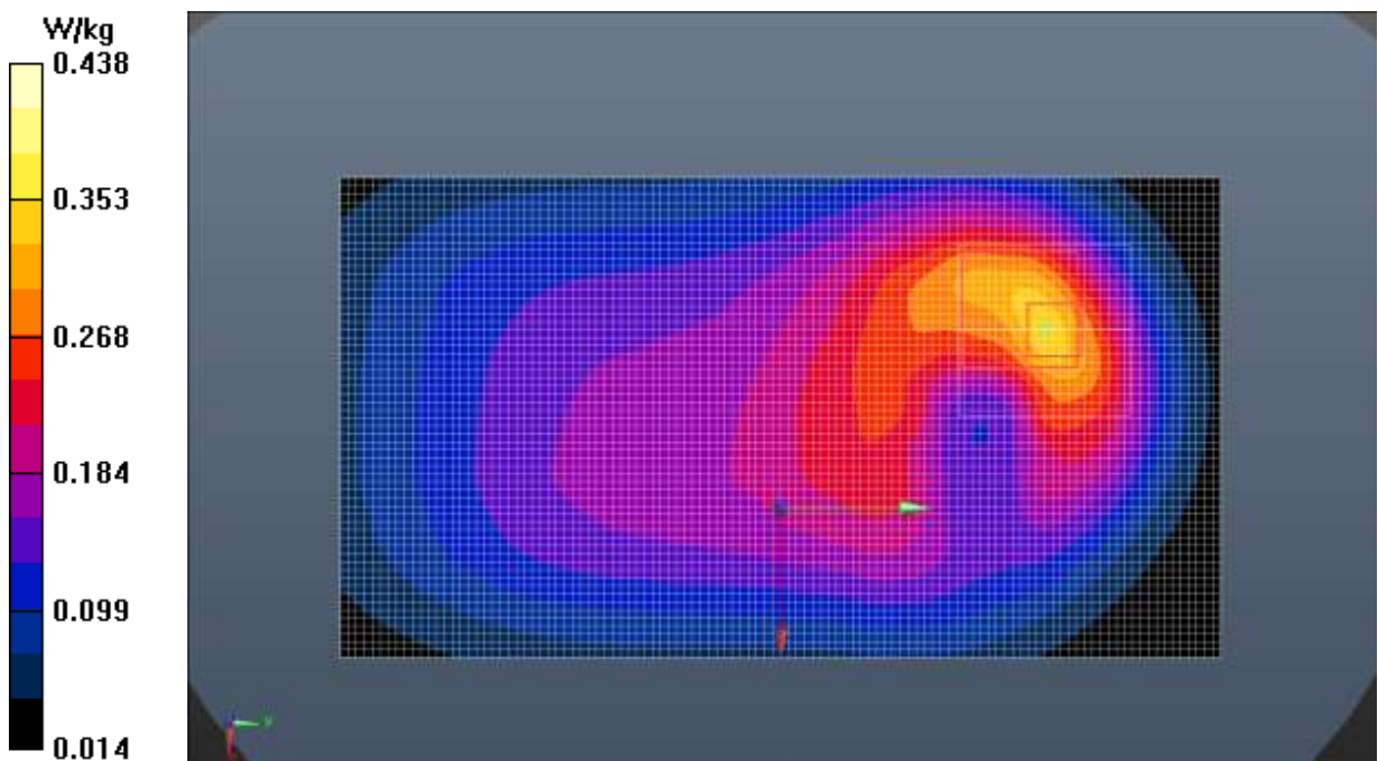
Fig.28 LTE Band 13
