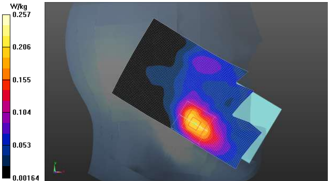
Fig.19 LTE Band 4
