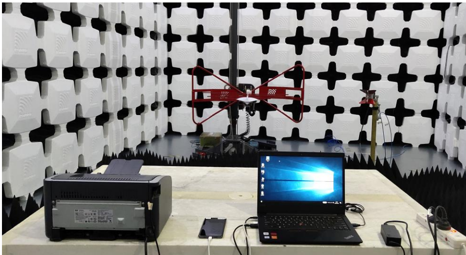
2. Radiated Emissions (Part 15B PC mode)( 1GHz-18GHz)
