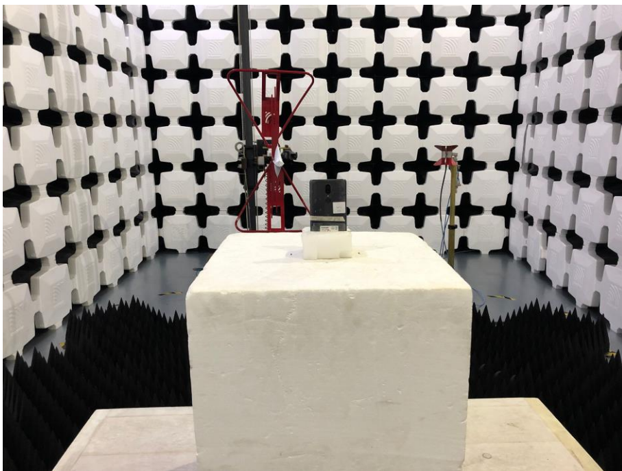
10. Radiated Emissions (Part 22/24/27/90) (30MHz-18GHz)
