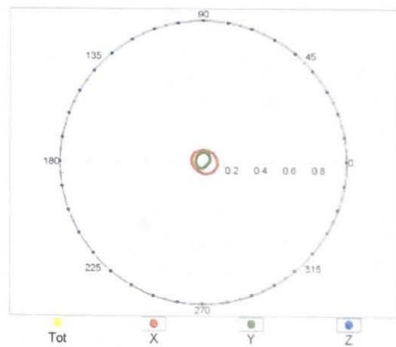
f=2500 MHz,R22,90°
