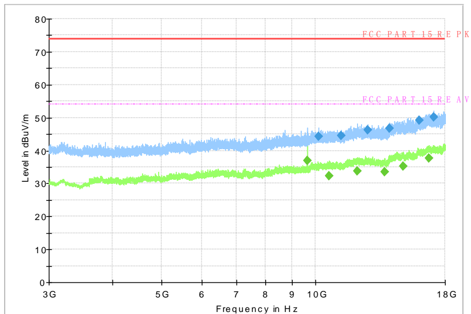
Fig.23 Radiated Spurious Emission (GFSK, Ch19, 3 GHz ~18 GHz)
