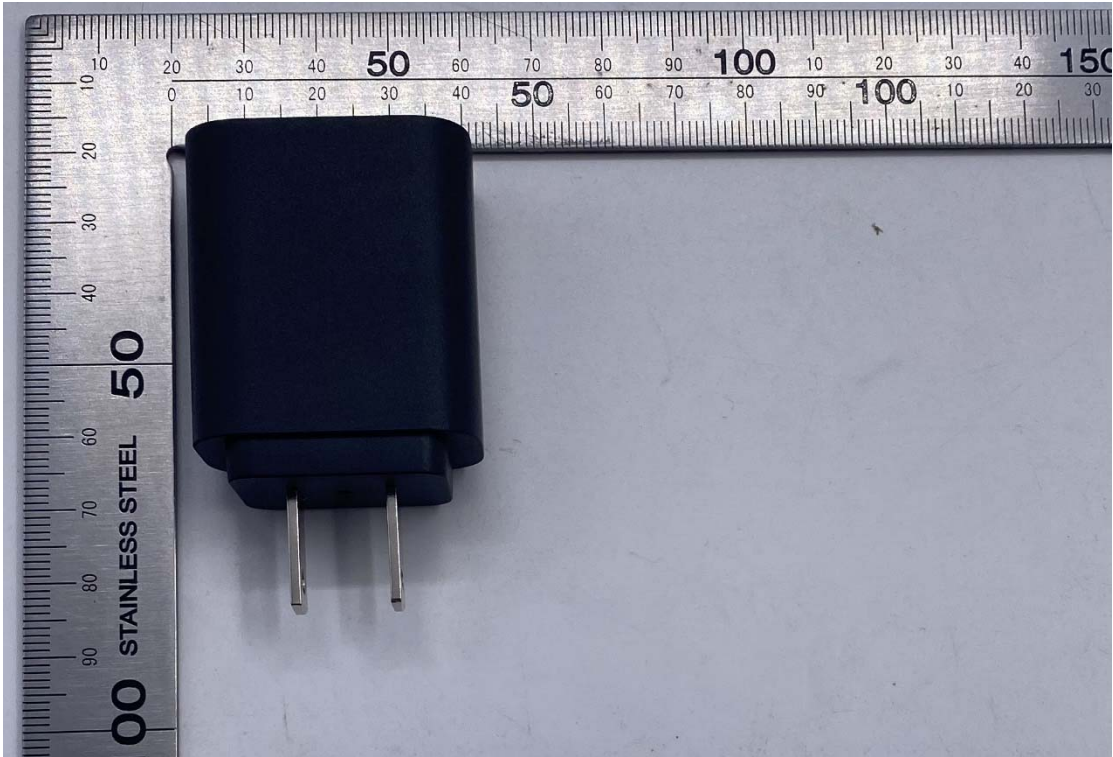
Charger View (Model: RD0502000-USBA-87MGmade by Ruide)
