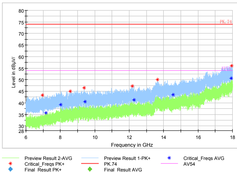
Pic7. Radiated emission (6GHz –18GHz)
