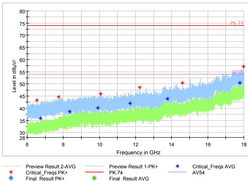
Pic11. Radiated emission (6GHz –18GHz)
