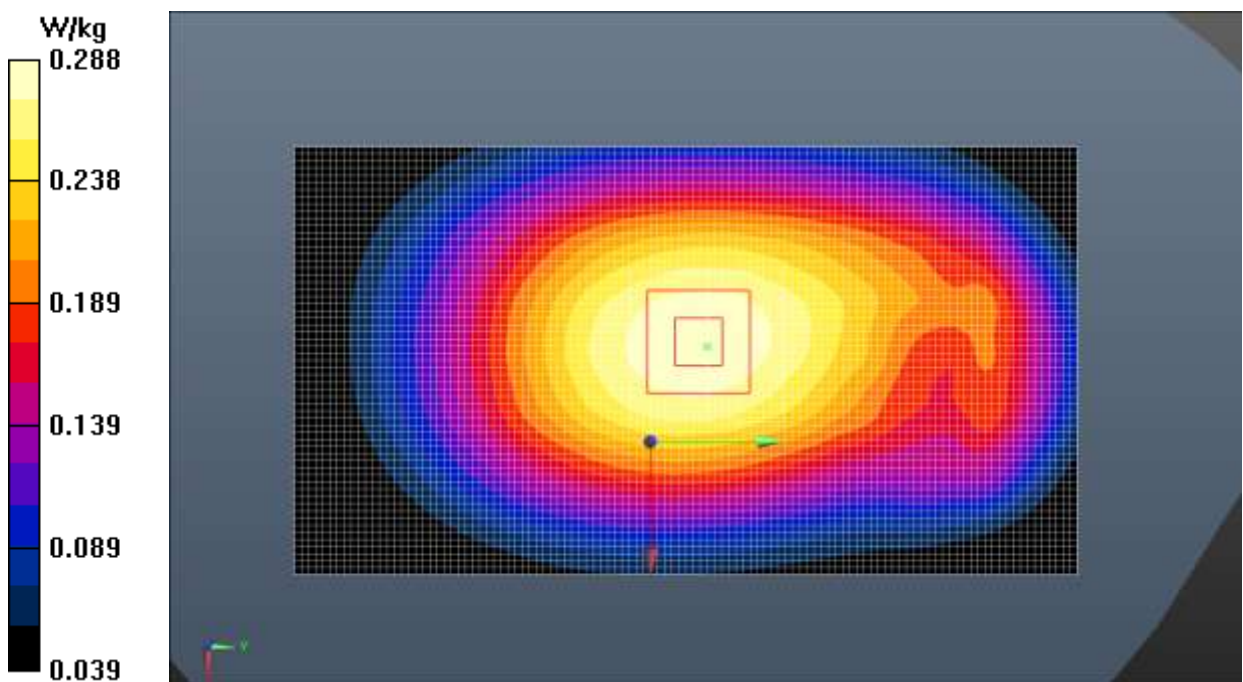
Fig.24 LTE Band 12
