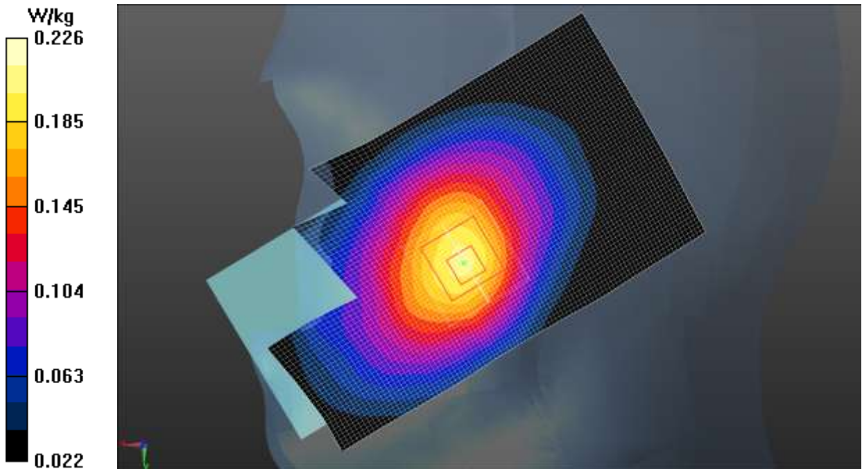
Fig.25 LTE Band 13
