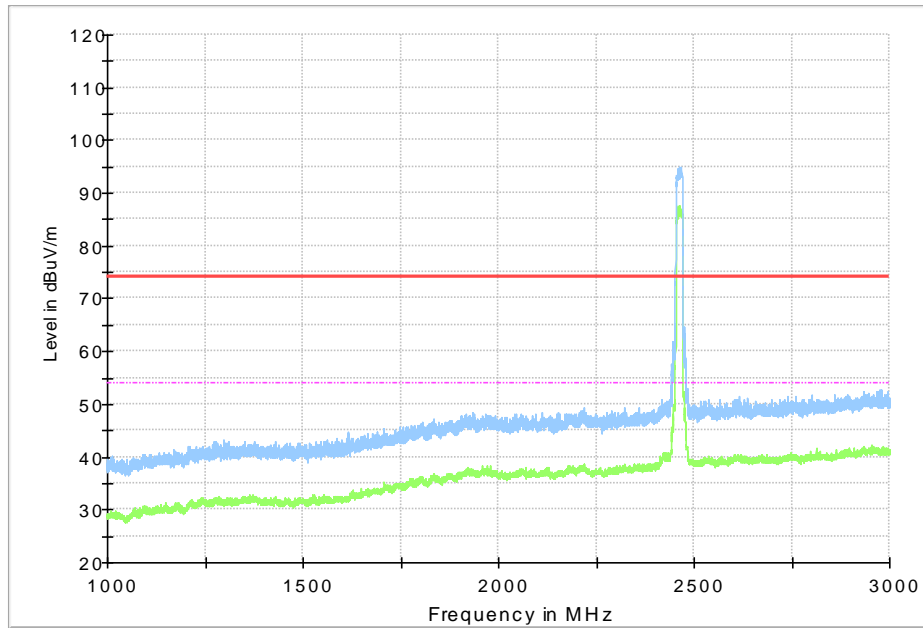
Fig.57 Radiated Spurious Emission (802.11g, CH11, 1GHz-3GHz)
