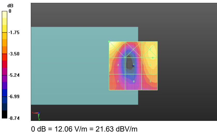
Fig A.7 HAC RF E-Field LTE-Band 41 High
