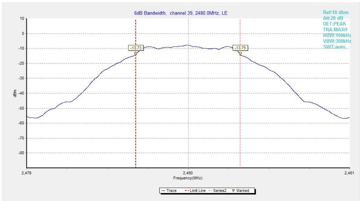
Fig.6 6dB Bandwidth (Ch 39), 1M
