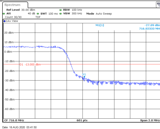
Band17-10MHz-QPSK-23780-1RB#49
