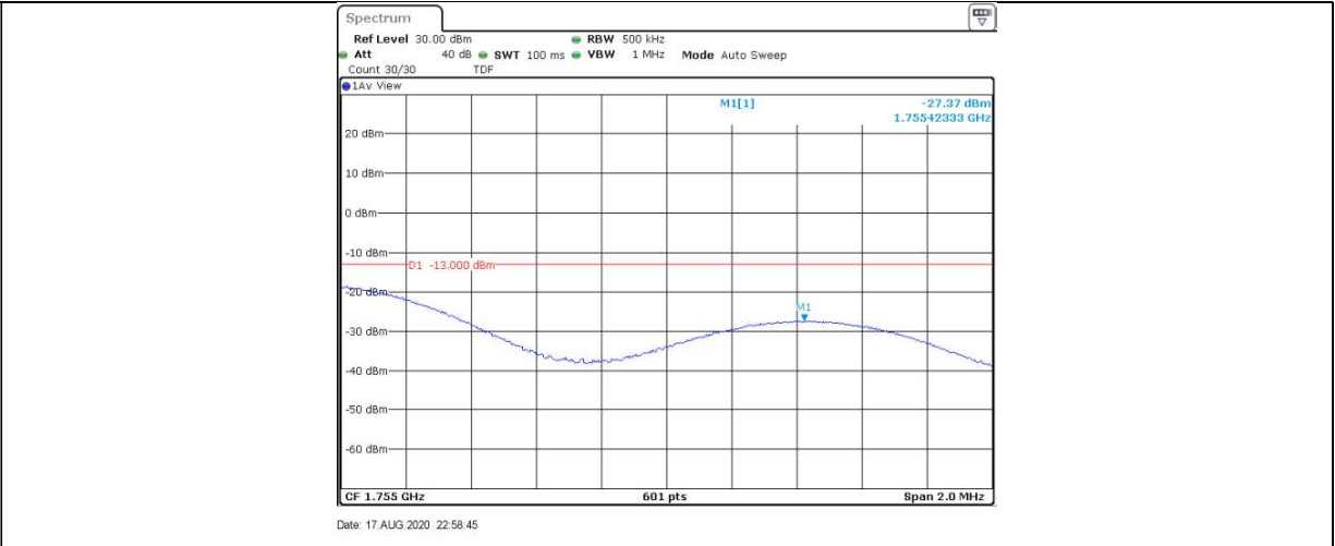
Band4-20MHz-QPSK-20300-100RB#0
