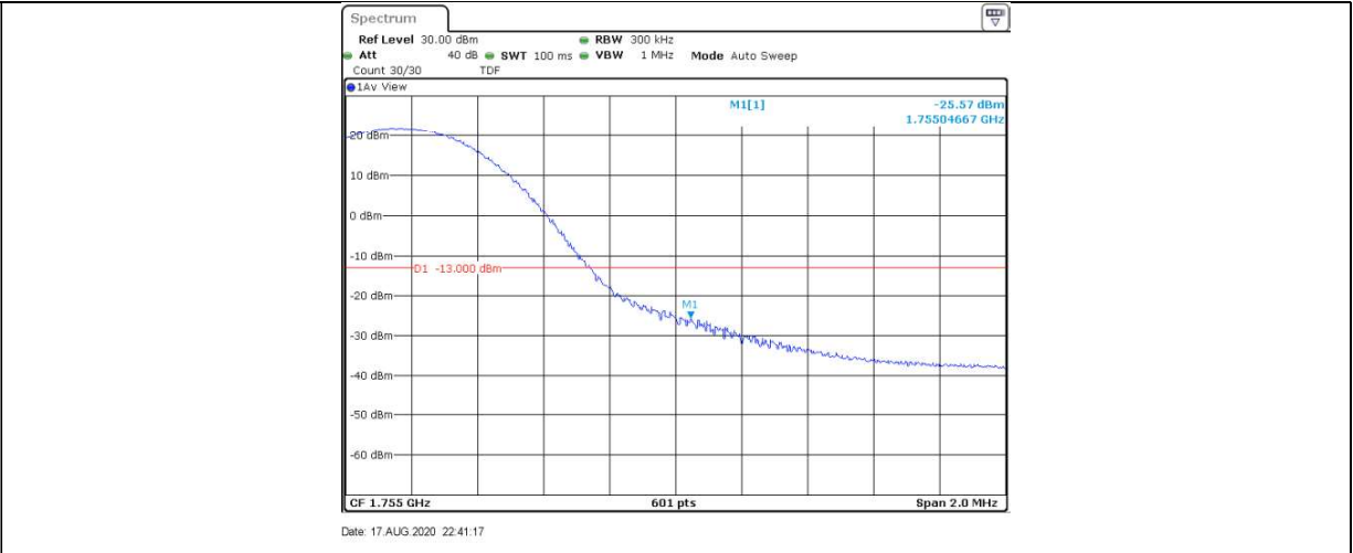
Band4-15MHz-QPSK-20325-75RB#0
