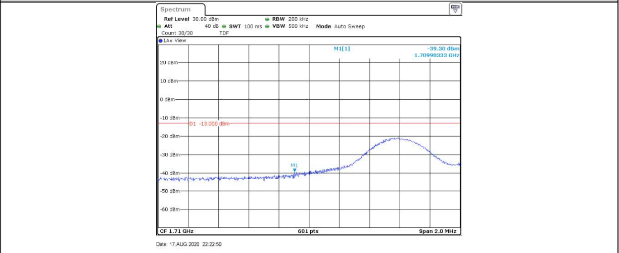
Band4-10MHz-QPSK-20350-50RB#0
