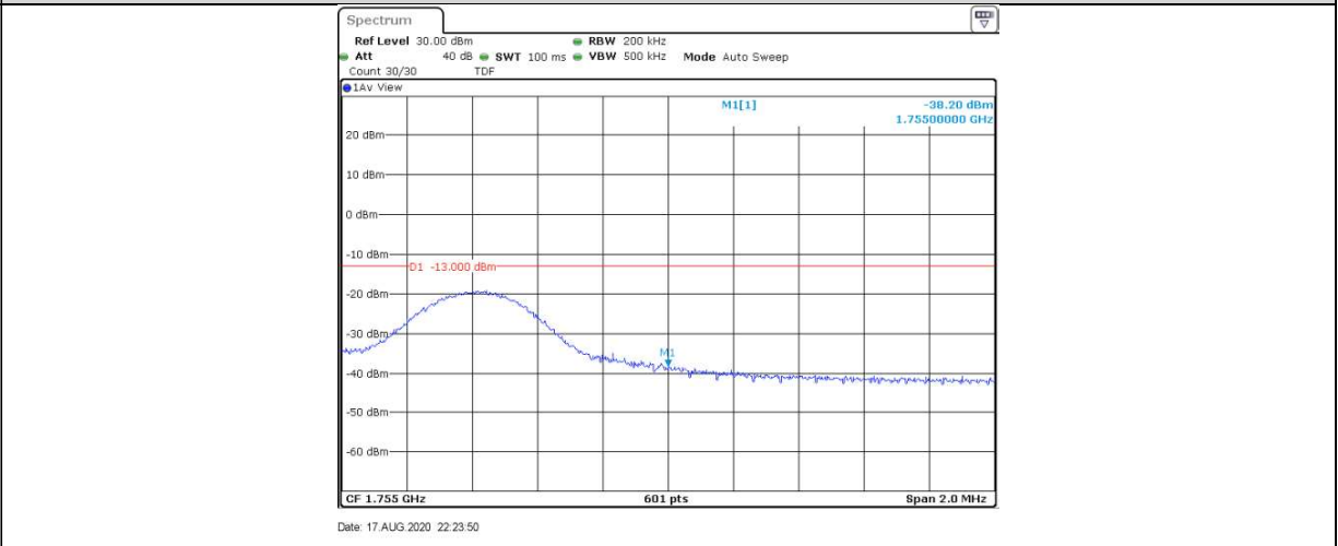
Band4-10MHz-16QAM-20350-1RB#49
