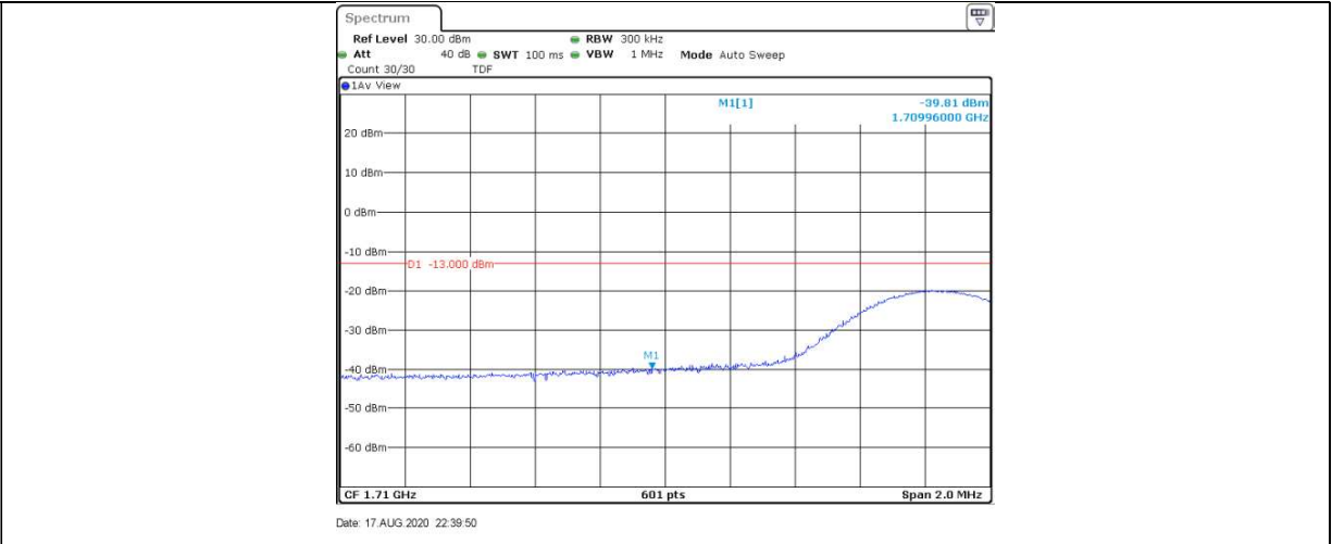
Band4-15MHz-QPSK-20025-75RB#0
