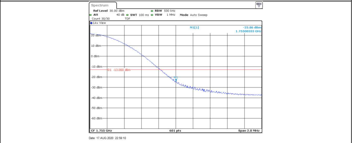
Band4-20MHz-QPSK-20300-1RB#0
