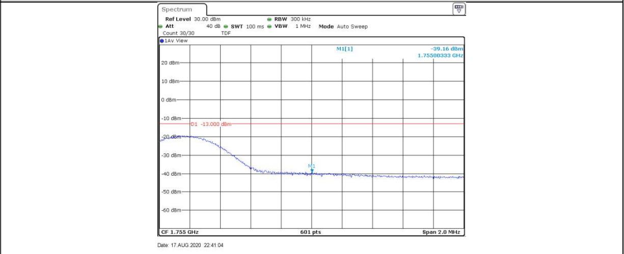
Band4-15MHz-16QAM-20325-1RB#74
